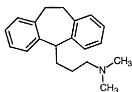
Imipramine (4c)
