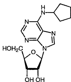
N 6 -Cyclopentyladenosine (56)
