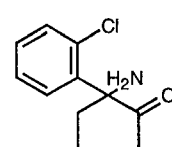
Norketamine (7)
