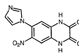
YM90K ( 22 )
