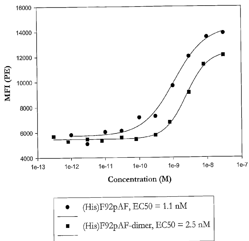
Figure 12 (His)F92pAF
