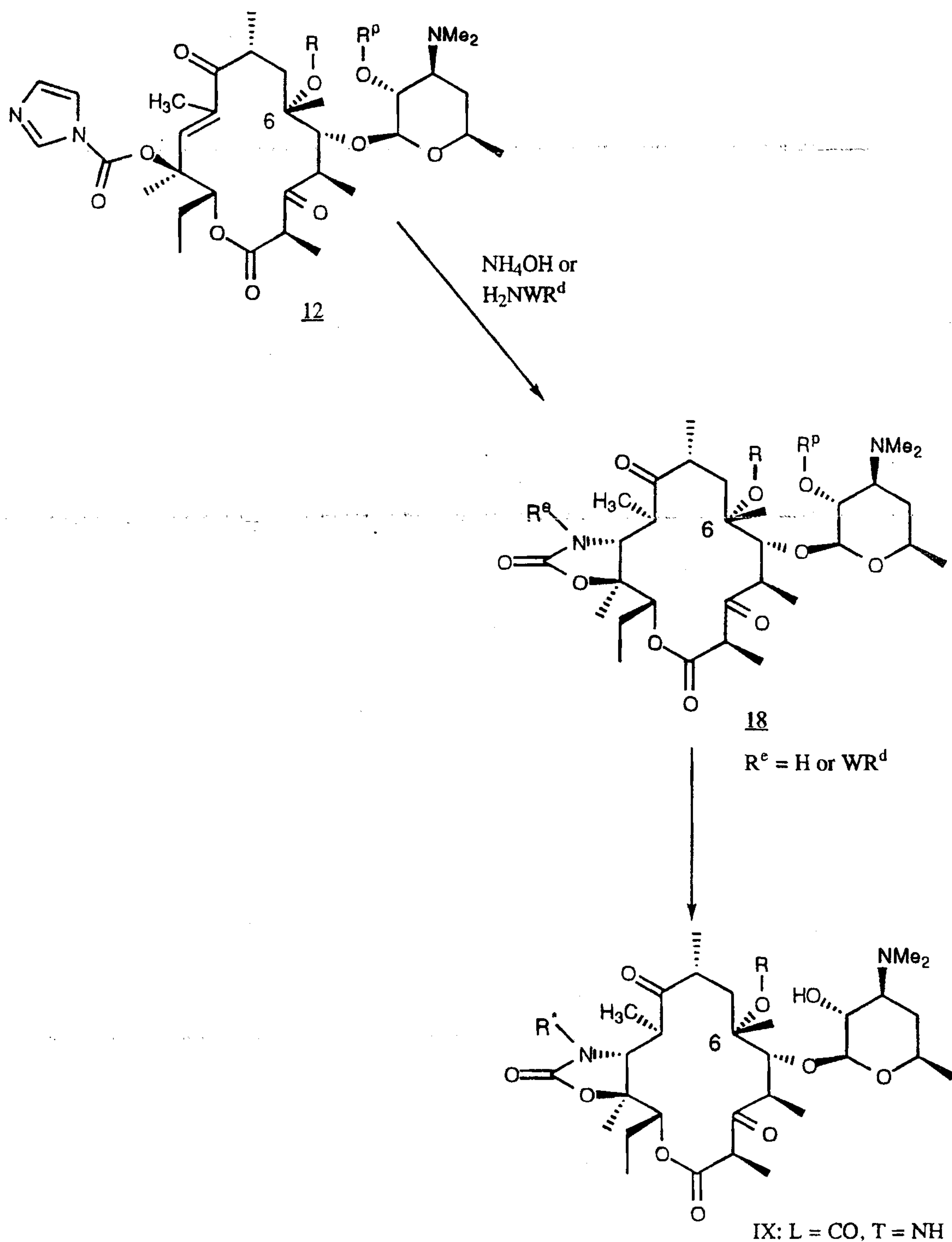
Scheme 4
