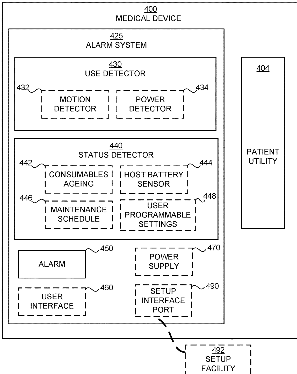
FIG. 4 MEDICAL DEVICE WITH ALARM SYSTEM
