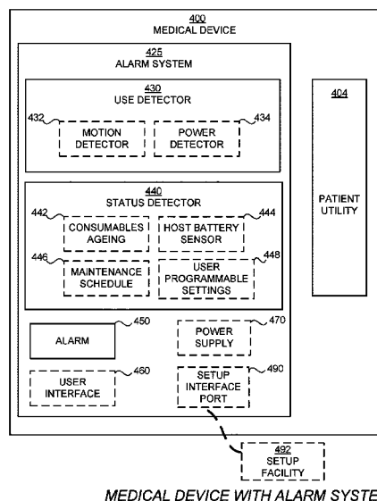
MEDICAL DEVICE WITH ALARM SYSTEM
