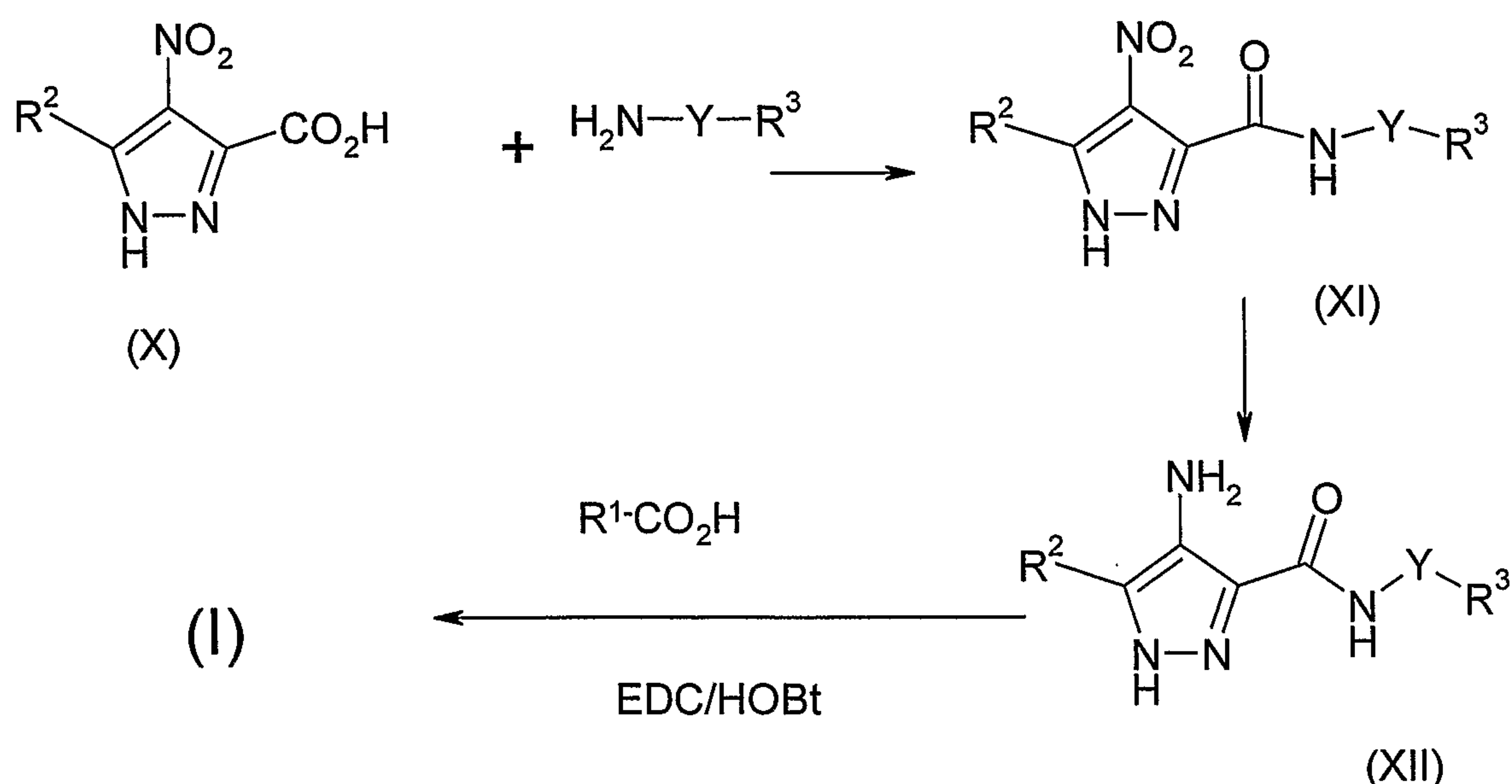
Scheme 1
