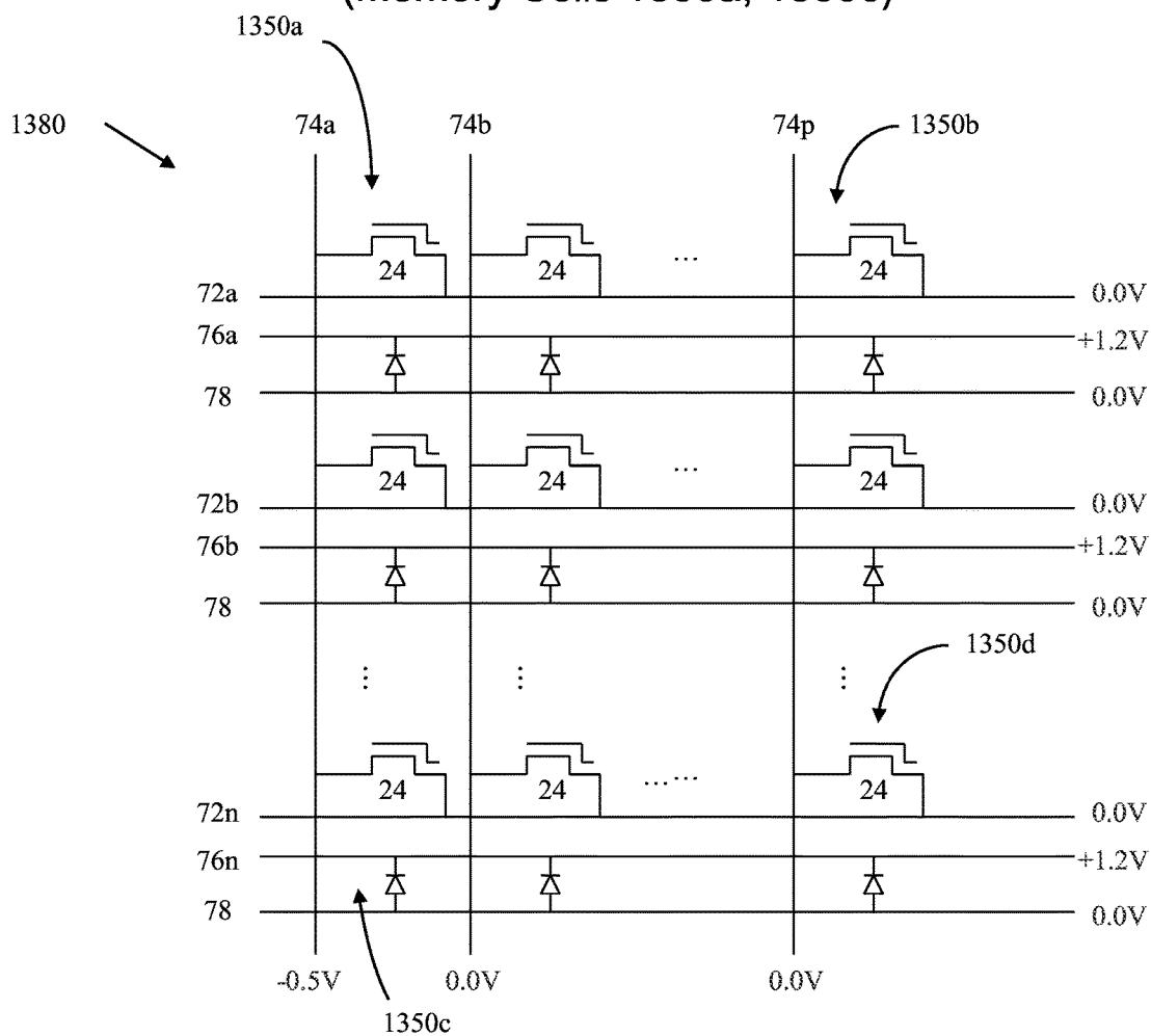
Write Logic-0 Operation (Memory Cells 1350a, 1350c)
