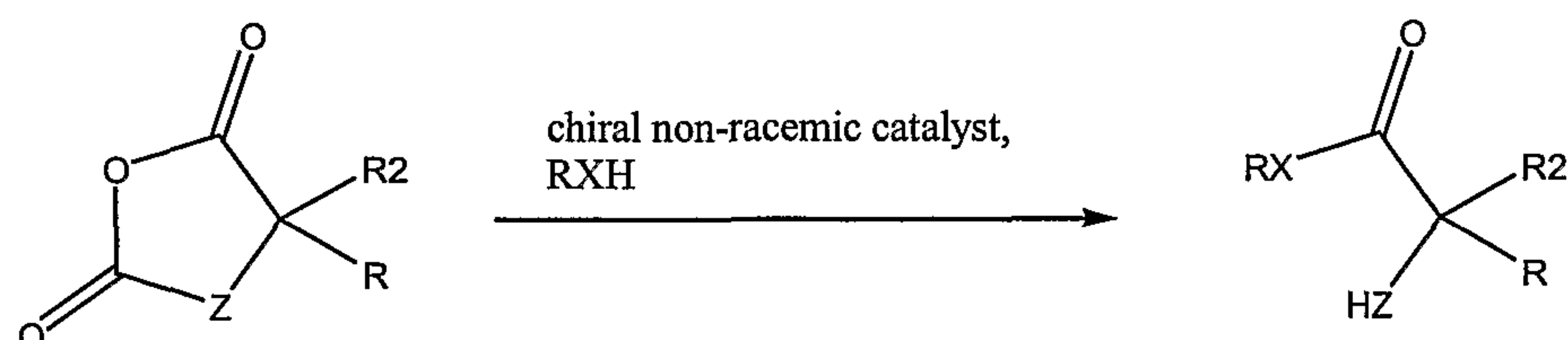
Scheme 2
