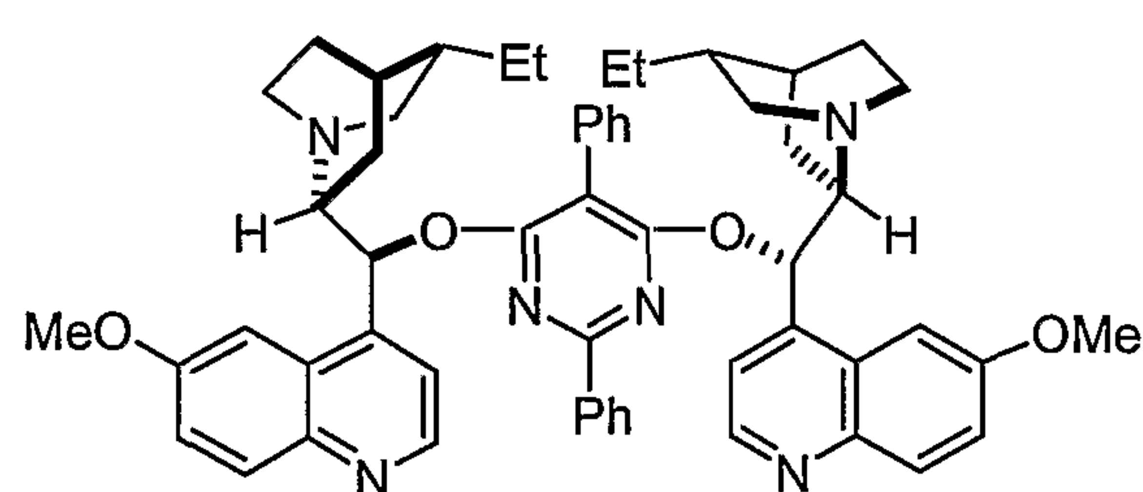
(DHQD) 2 PYR
