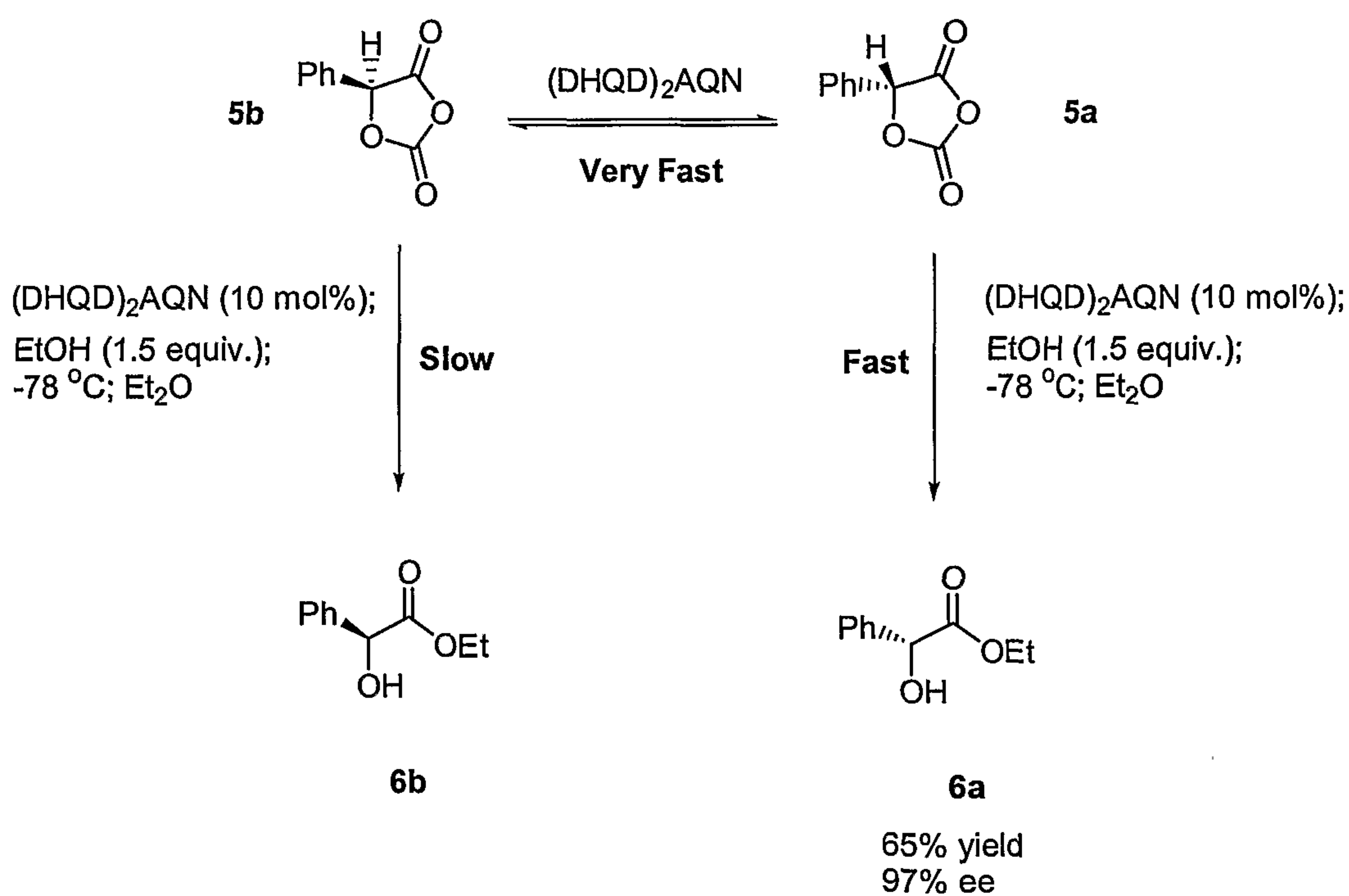
Scheme 2
