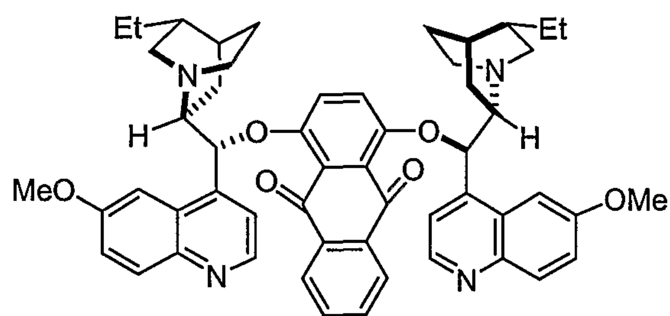
(DHQ) 2 AQN
