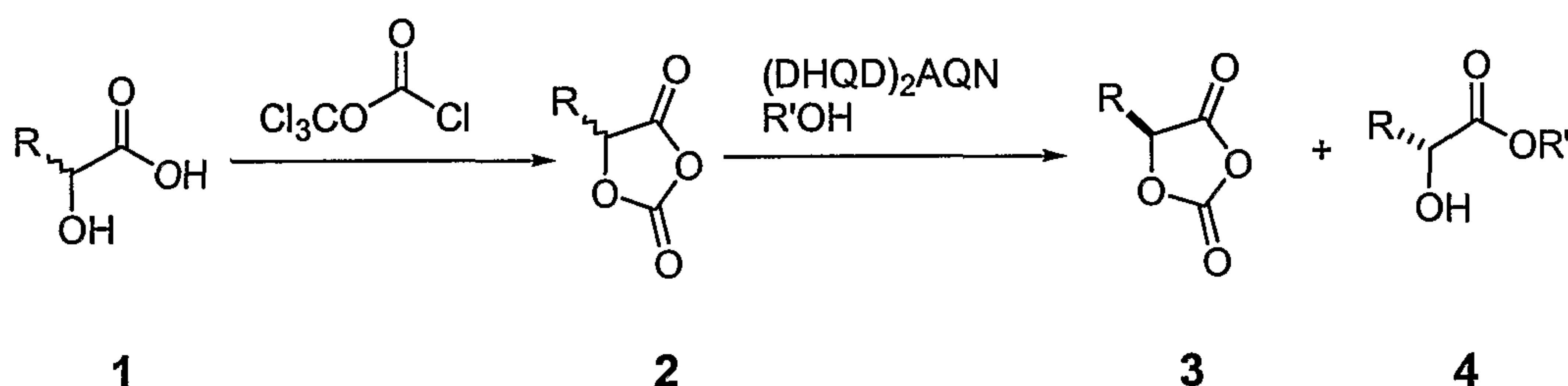
Scheme 1
