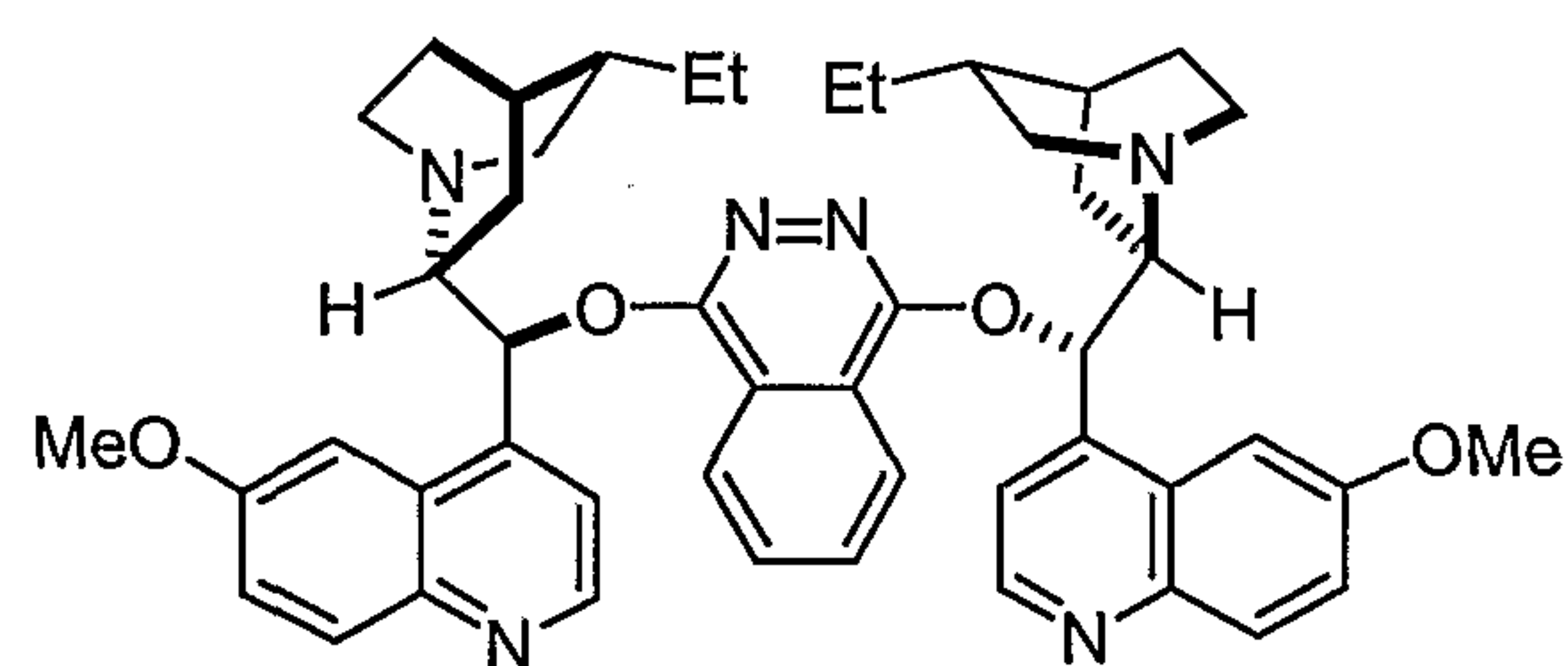
(DHQD) 2 PHAL
