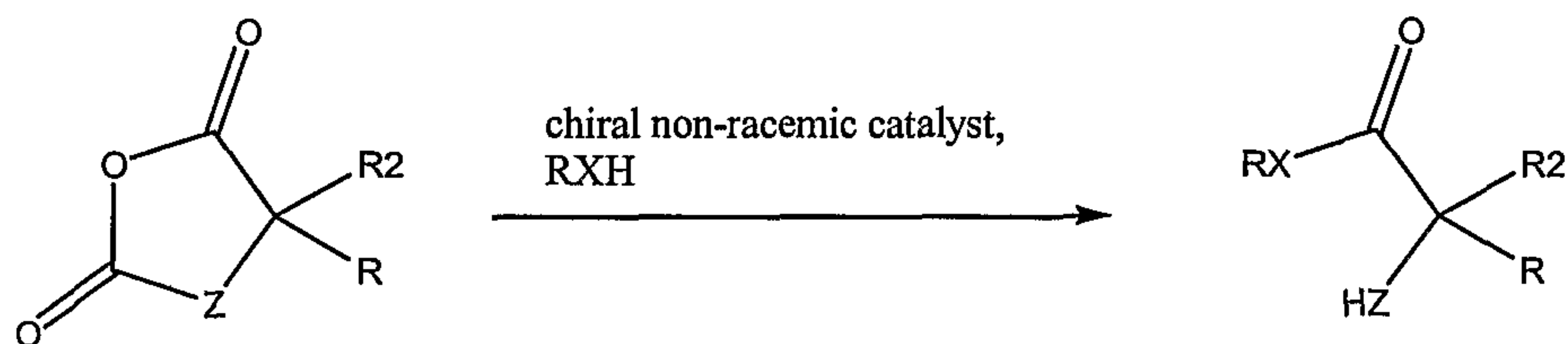
Scheme 2
