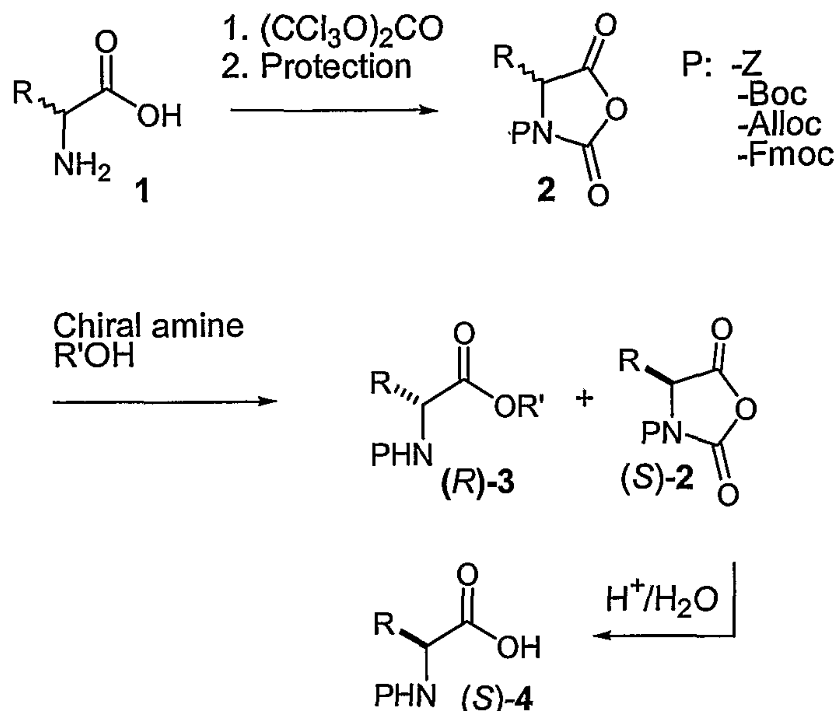
Scheme 3
