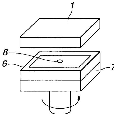
FIG.10C PRIOR ART
