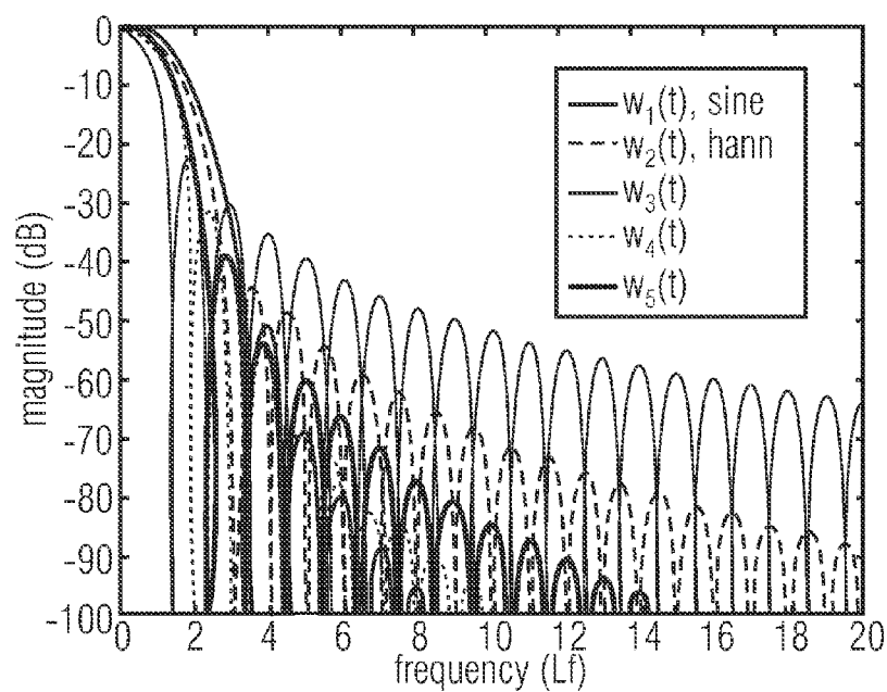
FIG 11 (SPECTRA OF SOME EXPONENTIATED SINE FUNCTIONS (12))
