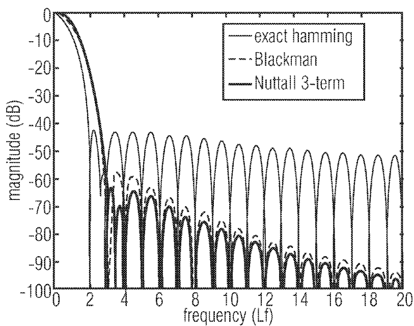
FIG 12 (SPECTRA OF OPTIMIZED SUM-OF-COSINES FUNCTIONS (15))
