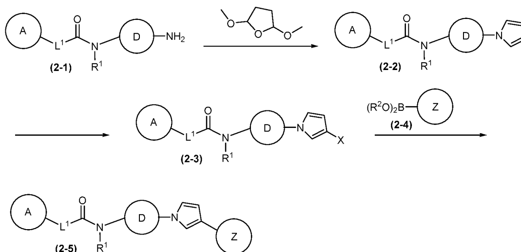
Scheme 2: Representative scheme for synthesis of exemplary compounds of the invention.
