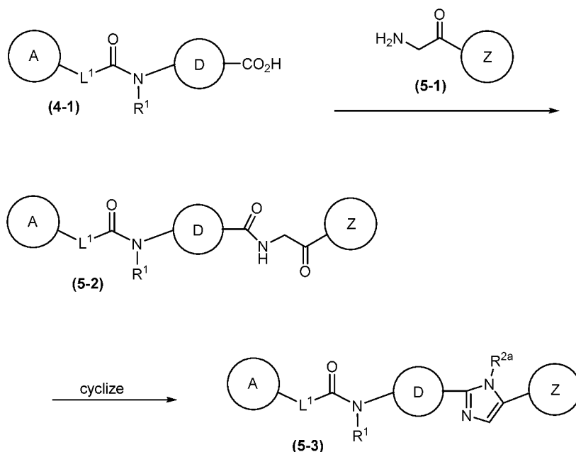
Scheme 5: Representative scheme for synthesis of exemplary compounds of the invention
