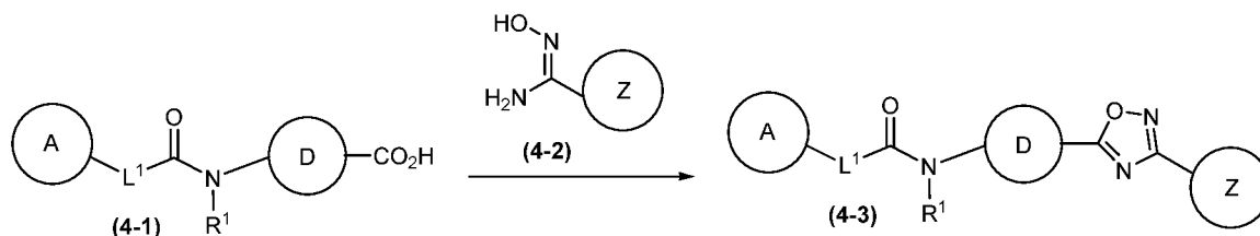
Scheme 4: Representative scheme for synthesis of exemplary compounds of the invention.
