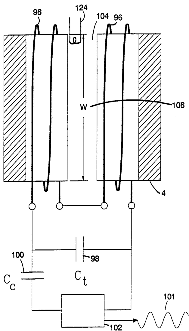
POWER AMPLIFIER
