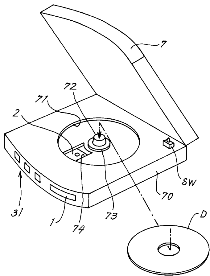
FIG .10 PRIOR ART
