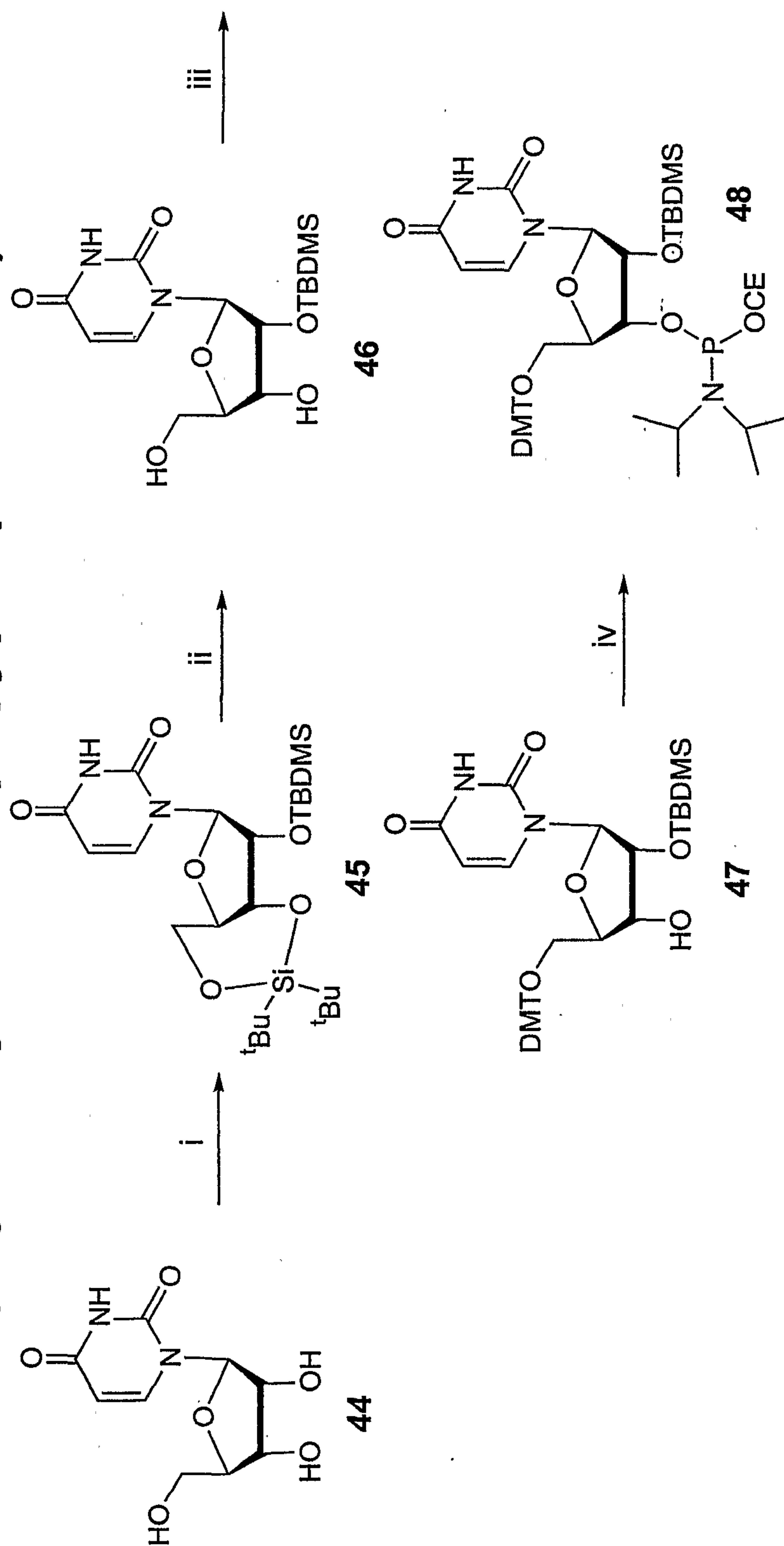
Figure 8: Synthesis of 5'-O-dimethoxytrityl-2'-O-tert-butyl-dimethylsilyl Uridine 3'-O-(2-cyanoethyl-N,N-diisopropylphosphoramidite)
