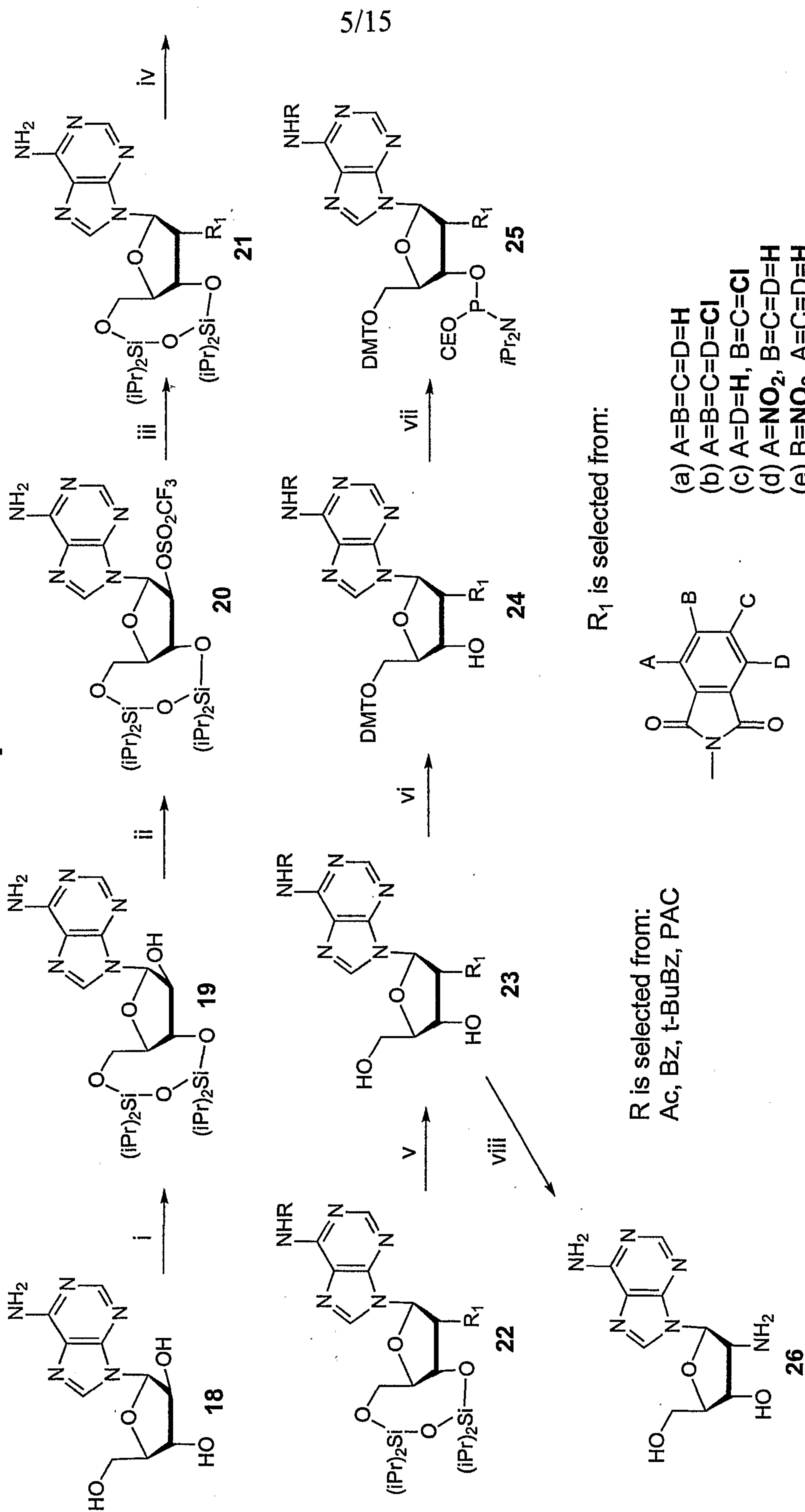
Figure 5: Synthesis of 2'-deoxy-2'-N-phthaloyl Adenosine Phosphoramidite
