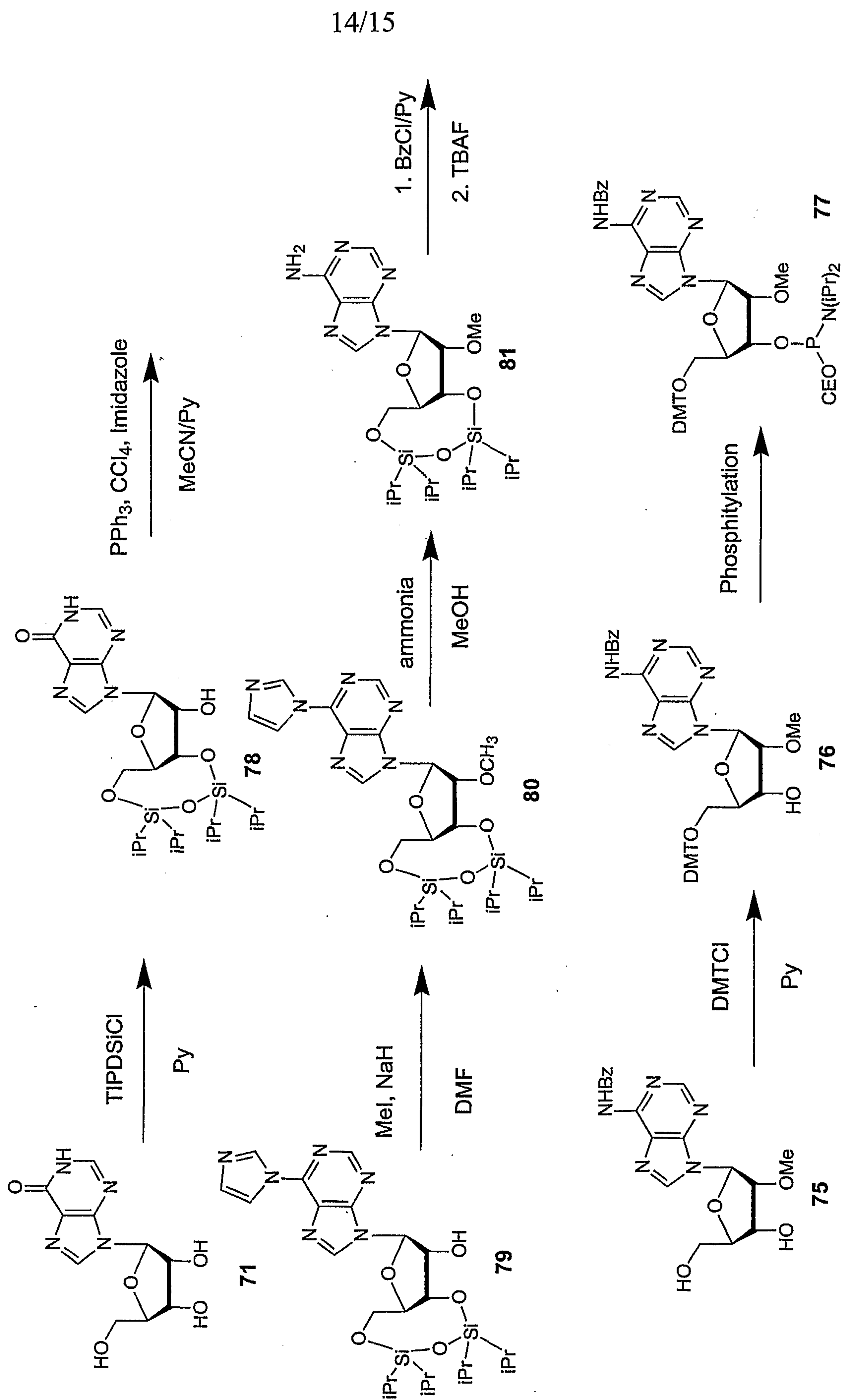
Figure 14: Synthesis of 2'-O-methyl Adenosine Derivatives
