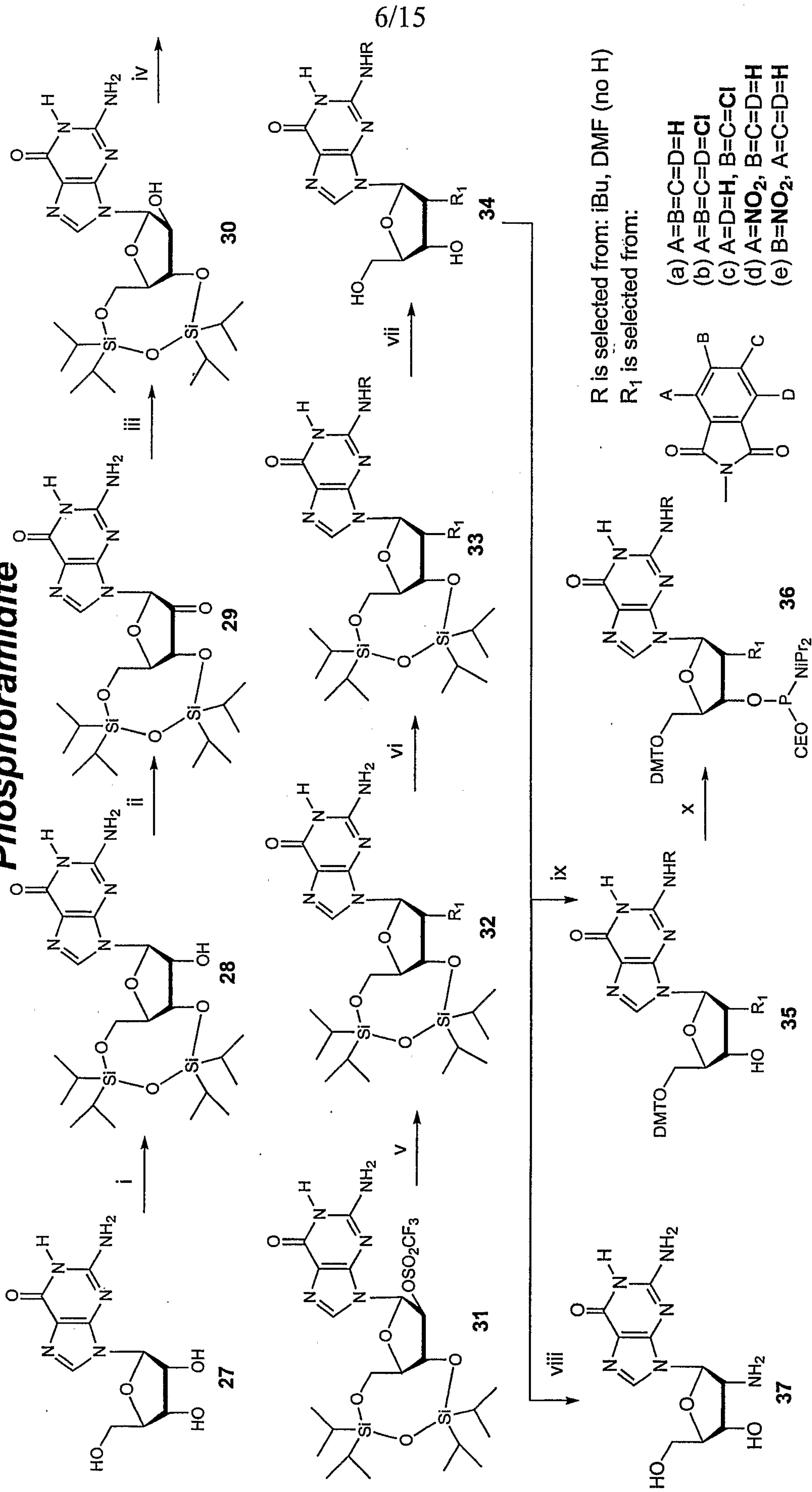
Figure 6: Synthesis of 2'-deoxy-2'-N-phthaloyl Guanosine
