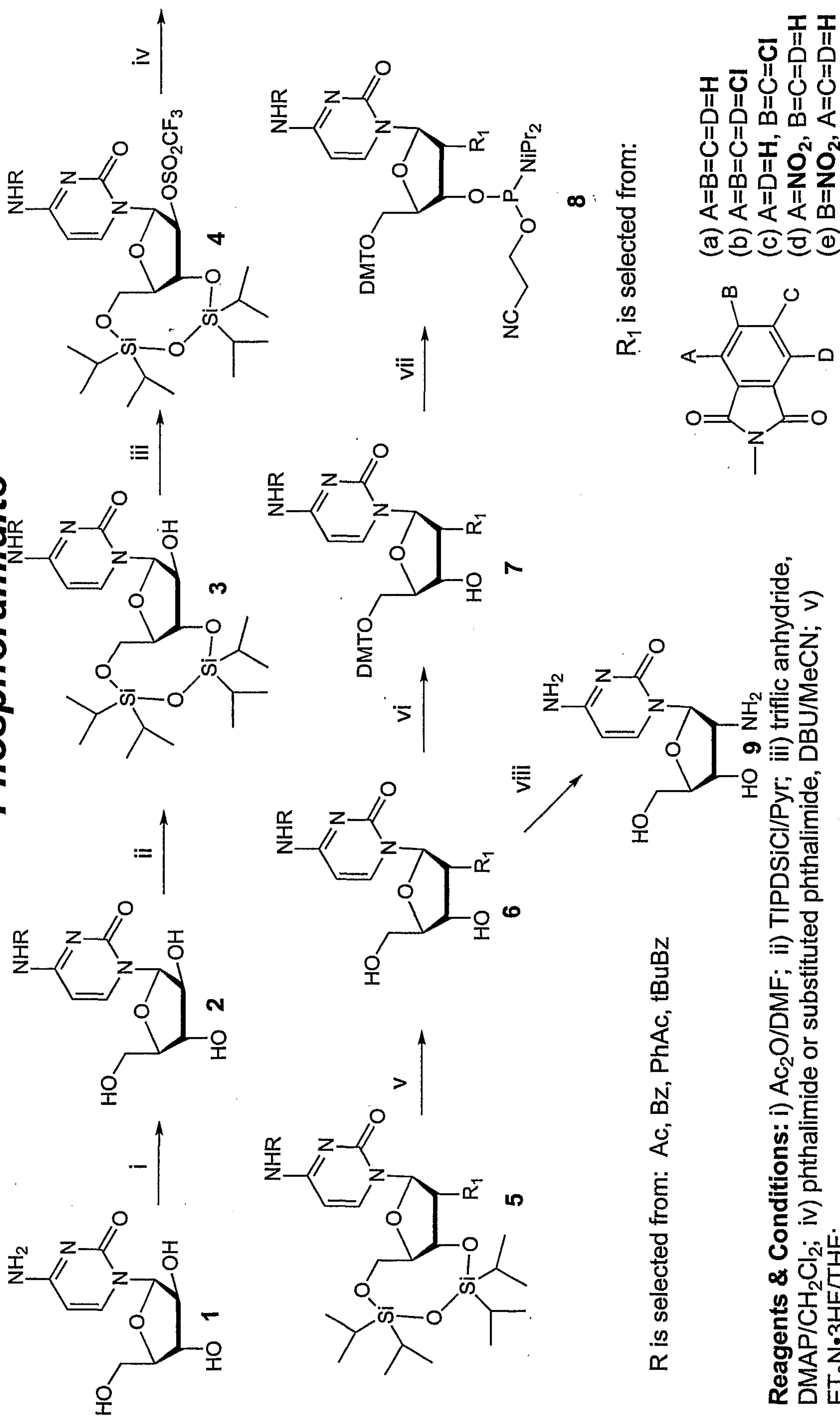
Figure 3: Synthesis of 2'-deoxy-2'-N-phthaloyl Cytidine
