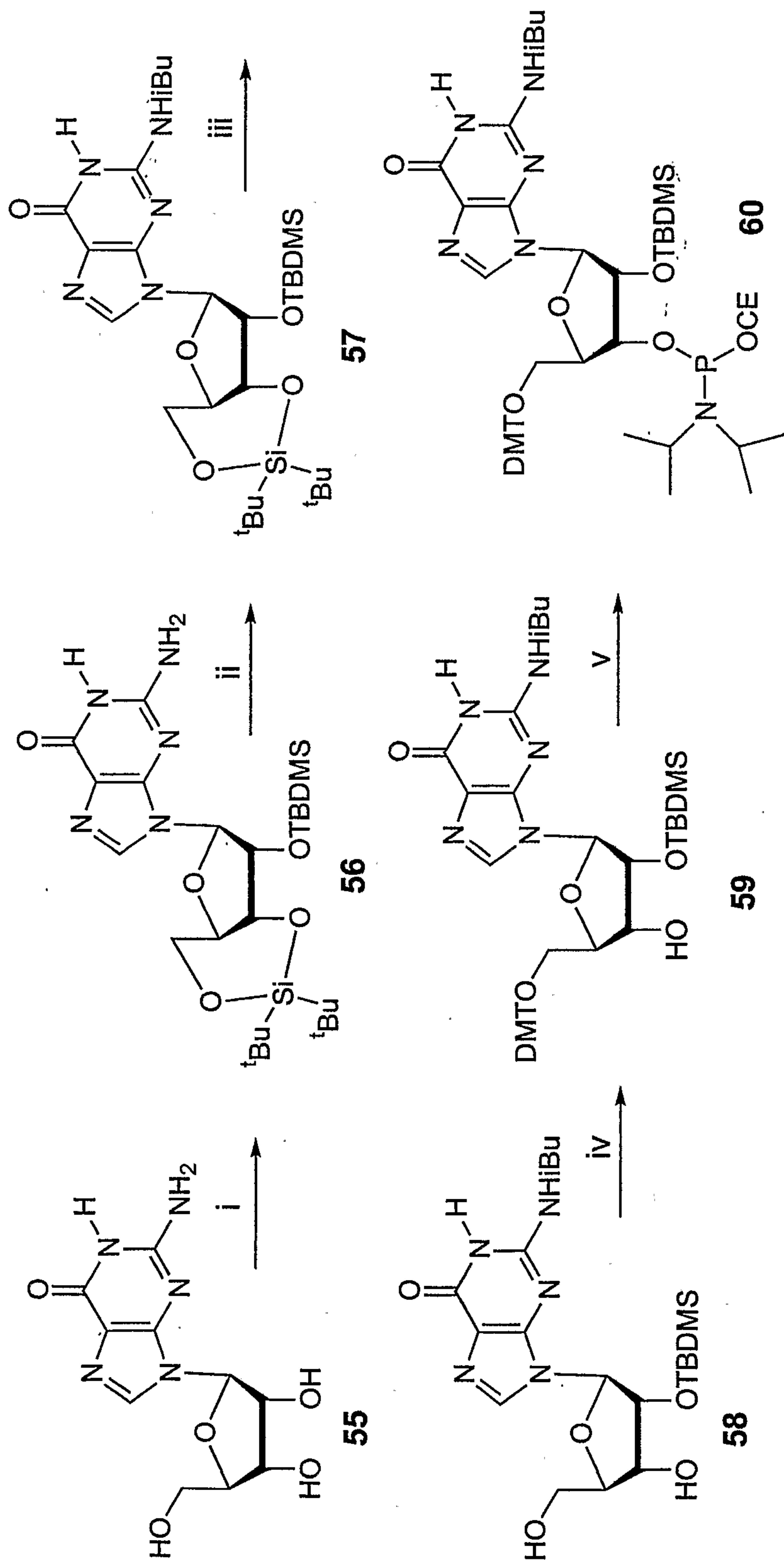
Figure 10: Synthesis of 5'-O-dimethoxytrityl-2'-O-tert-butylidimethylsilyl-N2-isobutyryl Guanosine 3'-O-(2-cyanoethyl-N,N-diisopropylphosphoramidite)
