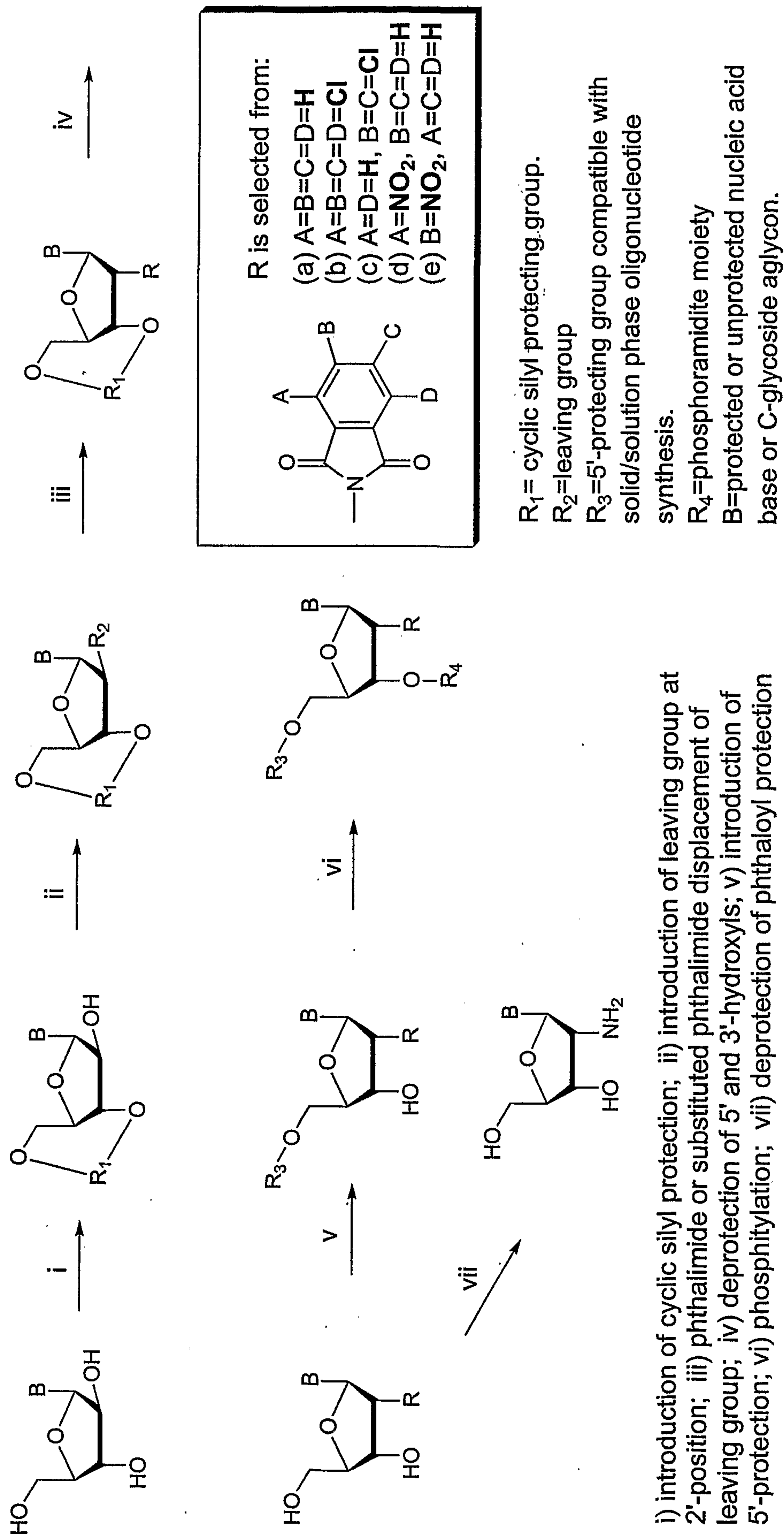
Figure 1: Synthesis of 2'-deoxy-2'-amino nucleosides, C-nucleosides and 2'-deoxy-2'-N-phthaloyl nucleoside and C-nucleoside phosphoramidites
