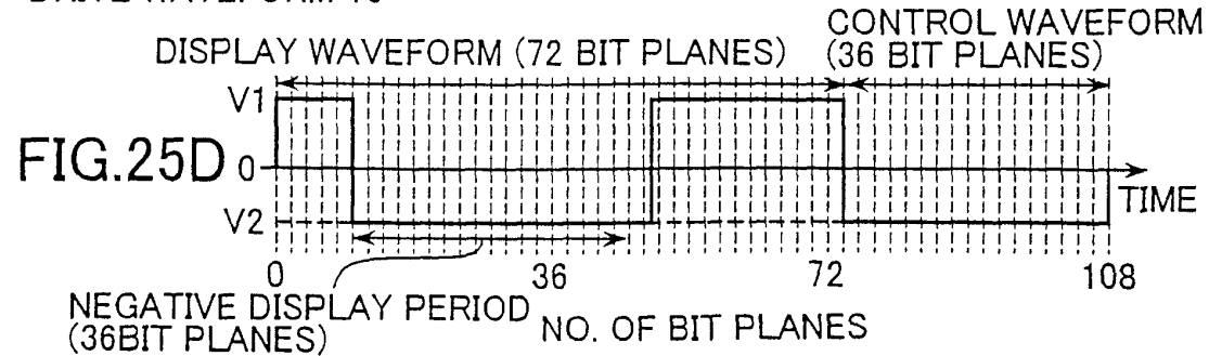
DRIVE WAVEFORM 16
