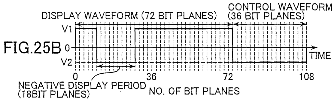
DRIVE WAVEFORM 14
