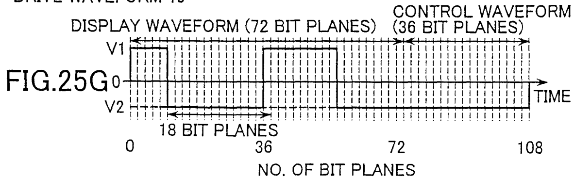
DRIVE WAVEFORM 19
