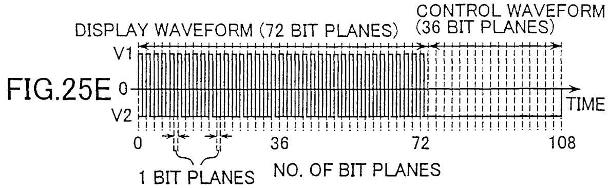
DRIVE WAVEFORM 17
