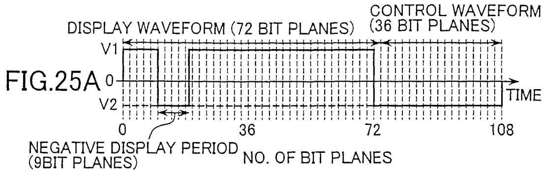
DRIVE WAVEFORM 13
