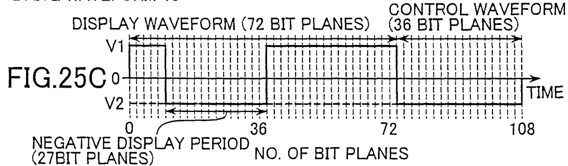
DRIVE WAVEFORM 15
