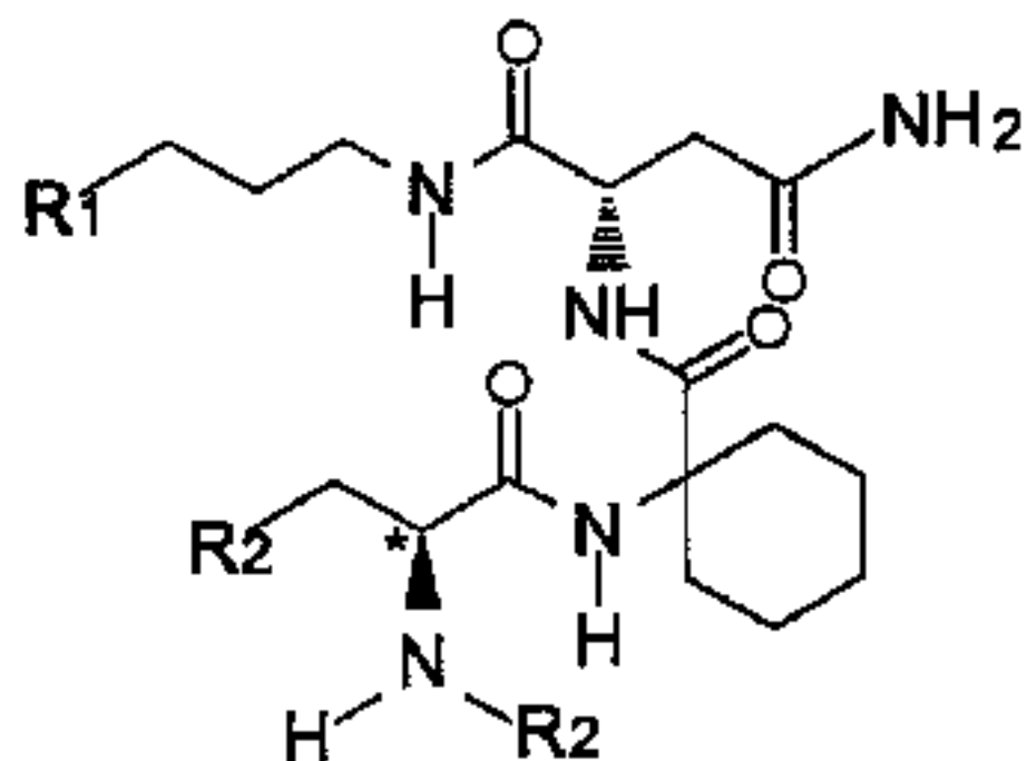
General Structure (*D, L and racemate claimed)
