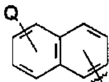
1 and 2-substitued naphthyl
