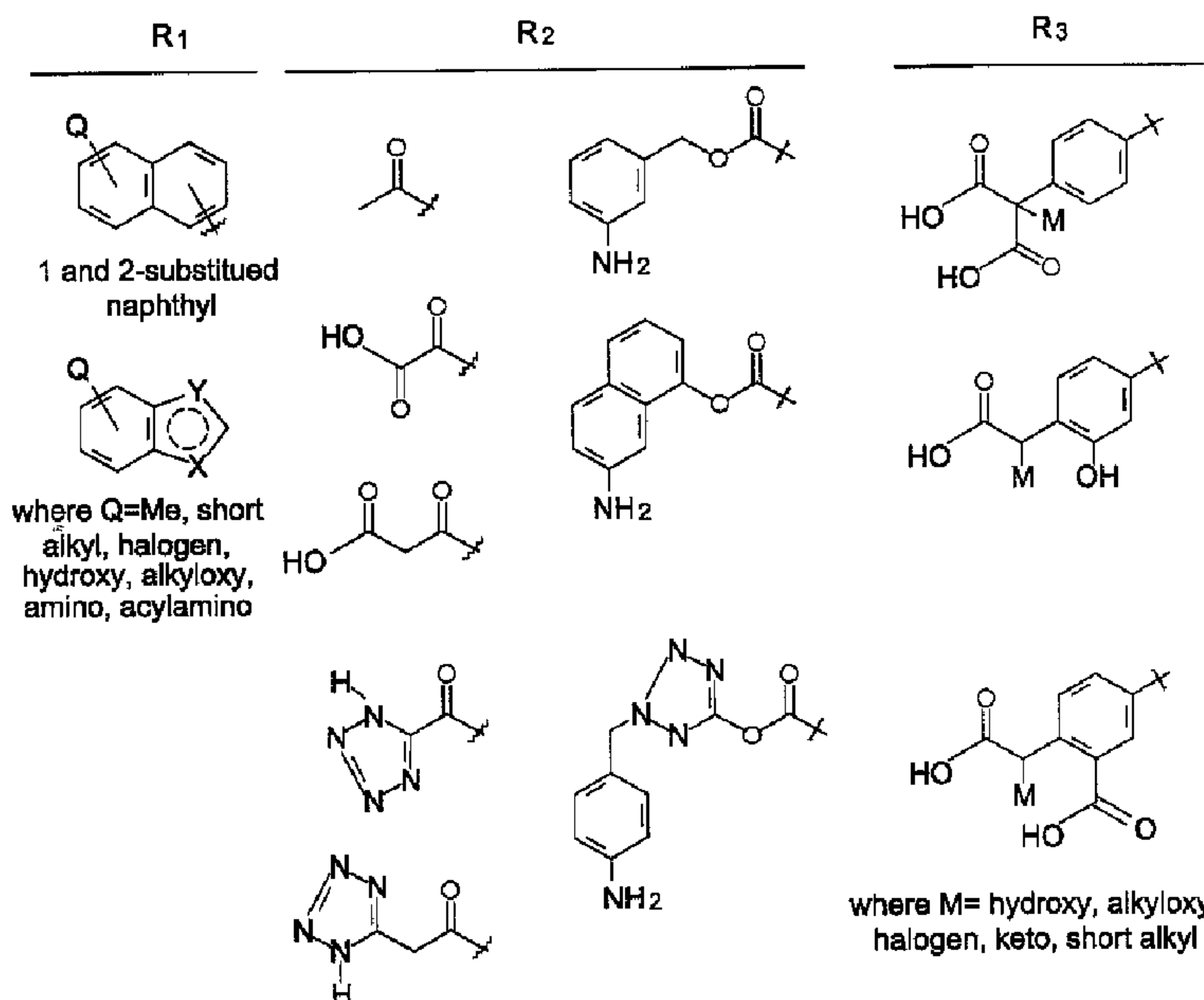
General Structure (*D, L and racemate claimed)
