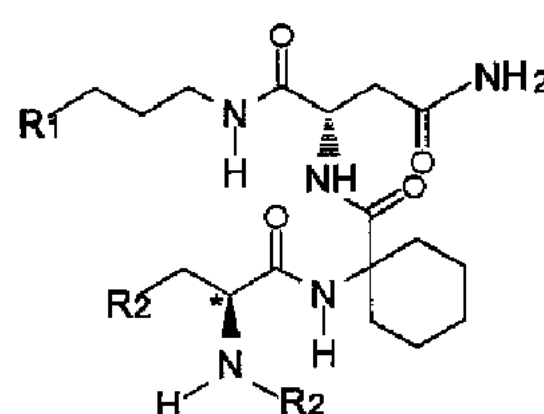
General Structure (*D, L and racemate claimed)
