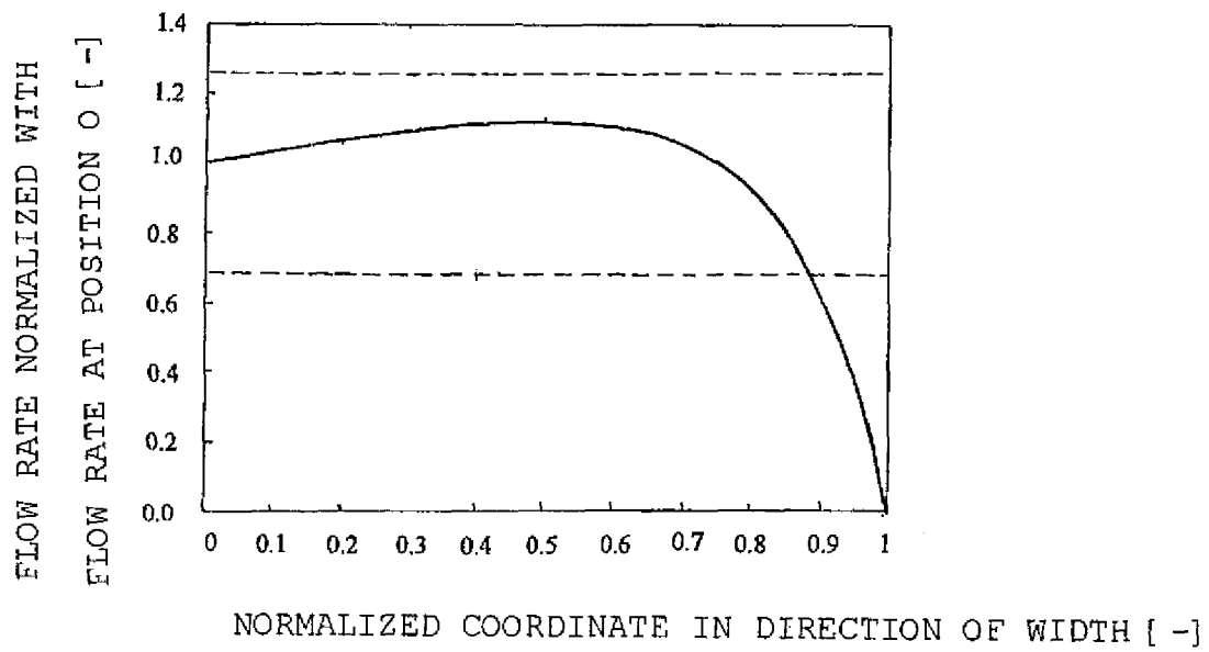
FLOW-RATE DISTRIBUTION WITHIN MANIFOLD IN EXAMPLES 1 TO 5
