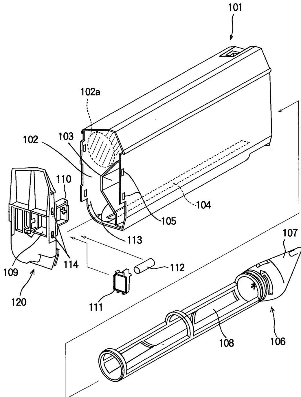
FIG.19 RELATED ART
