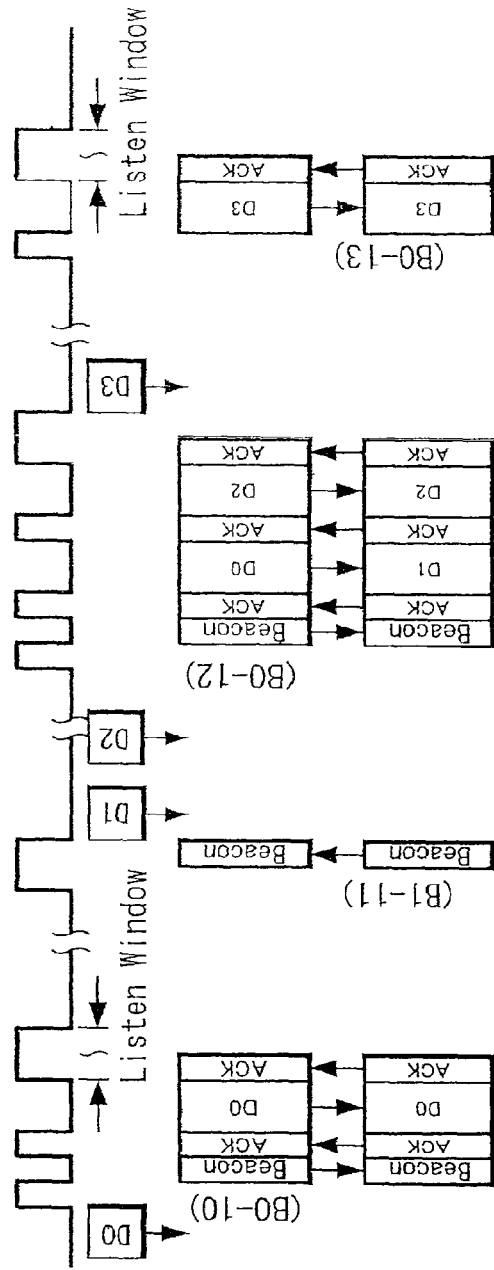
FIG. 16A STA-0 Rx State
