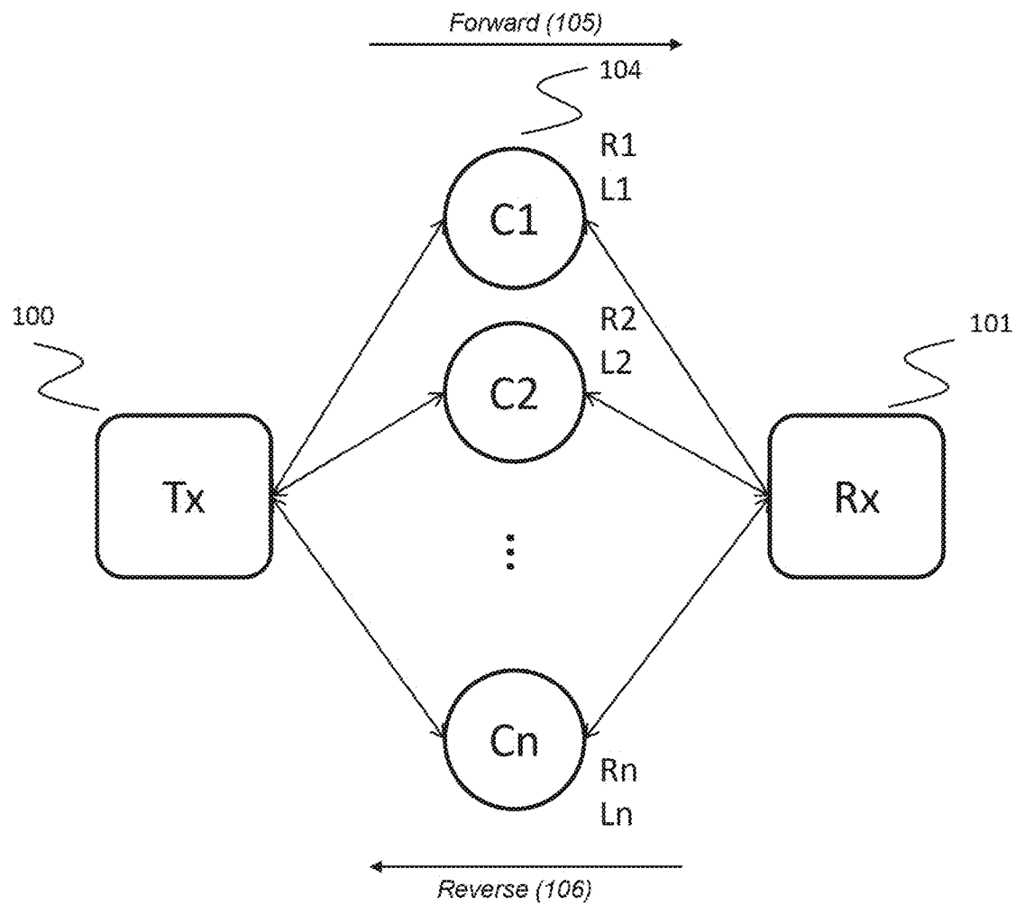
Figure 1. Bonded connections between transmitter and receiver
