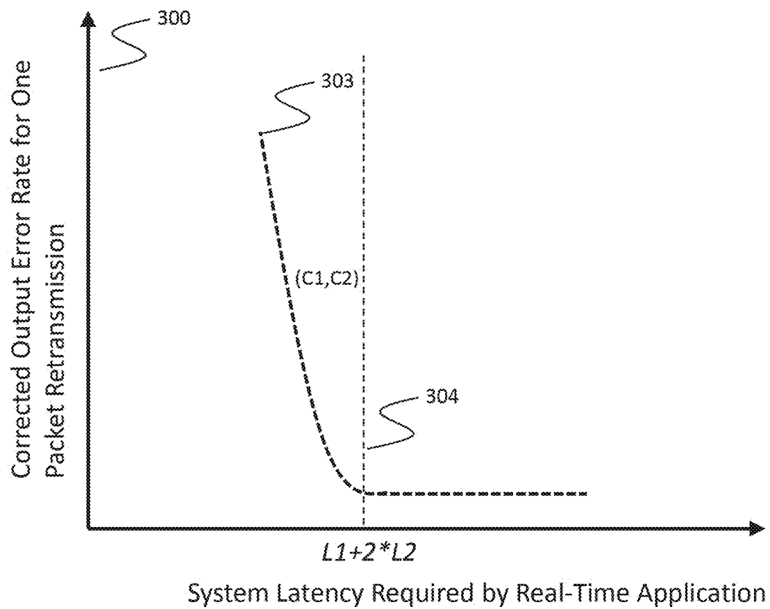
Figure 3. Combined Latency versus Output Error Rate
