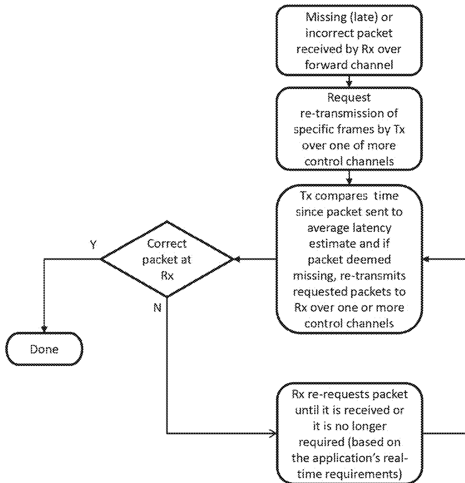
Figure 4. Error Correction via Packet Re-transmission
