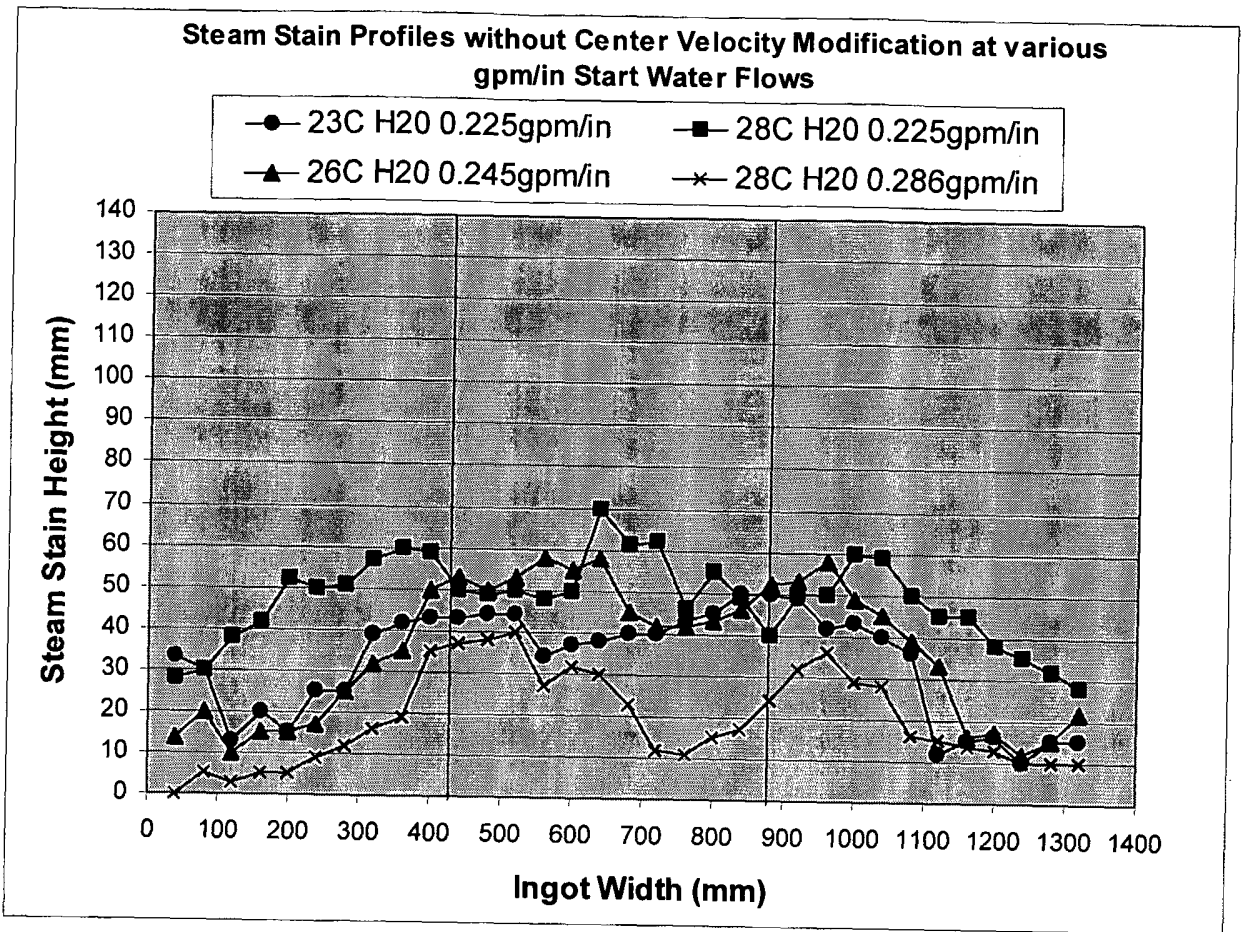
Steam Stain Measurements of 508x1524 ingots of 5083 before coolant stream velocity modification at varying water flow rates.
