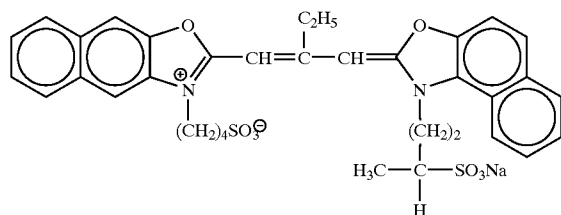
Sensitizing dye 5
