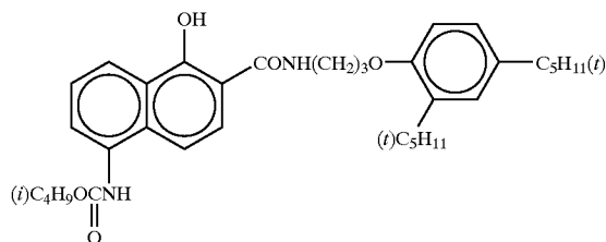
ExC-4
