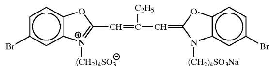
Sensitizing dye 5
