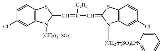
Sensitizing dye 3
