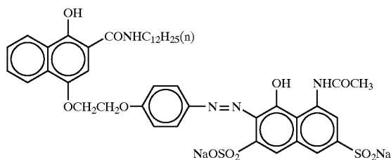
ExC-2
