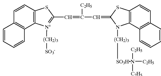
Sensitizing dye 4
