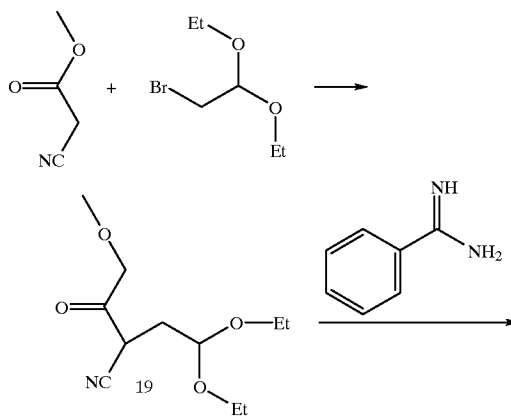
Scheme VIII
