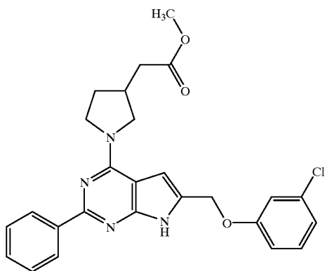
(Compound 1716)
