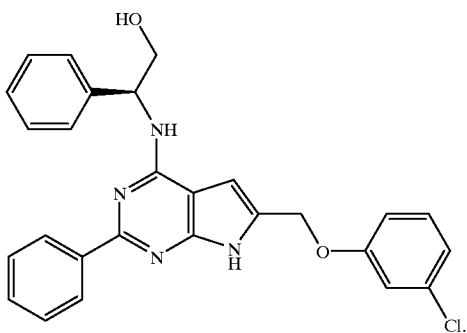
(Compound 1714)
