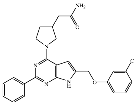
(Compound 1717)
