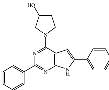
(Compound 1703)
