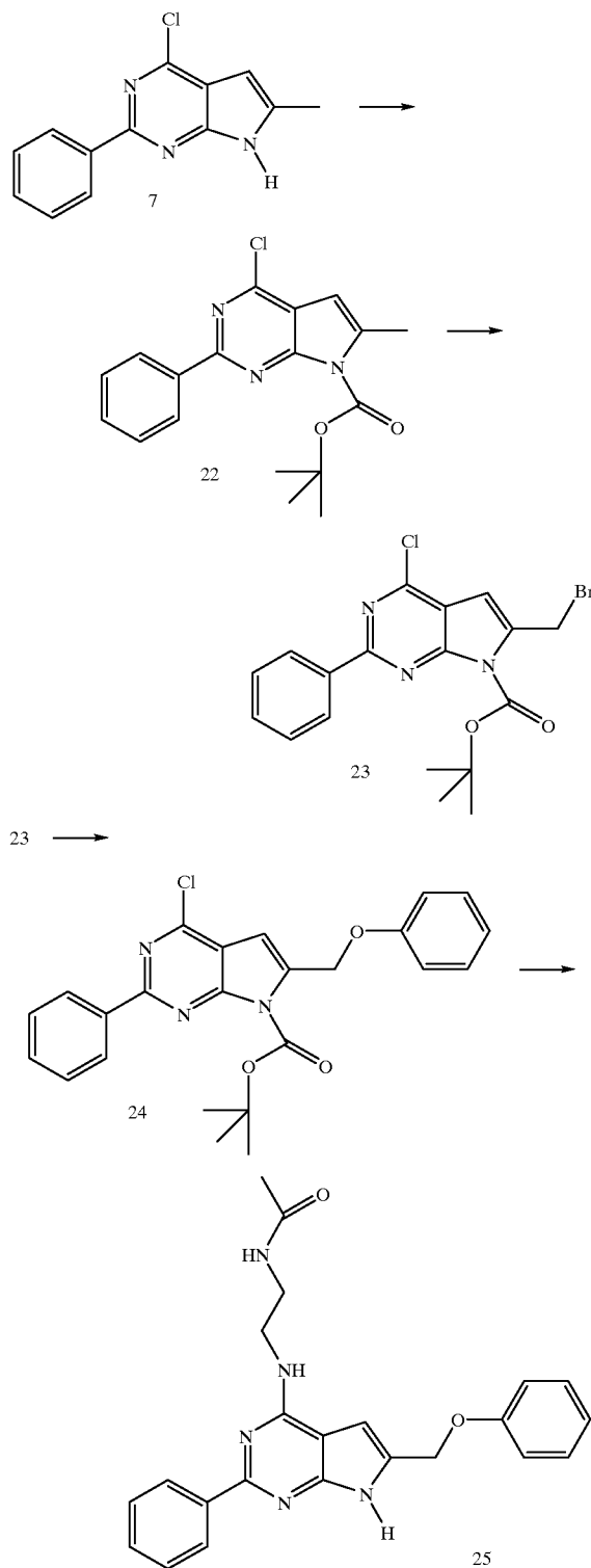
Scheme IX
