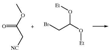
Scheme VII
