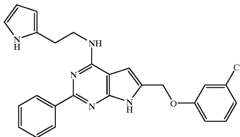
(Compound 1712)
