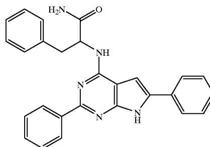
(Compound 1710)
