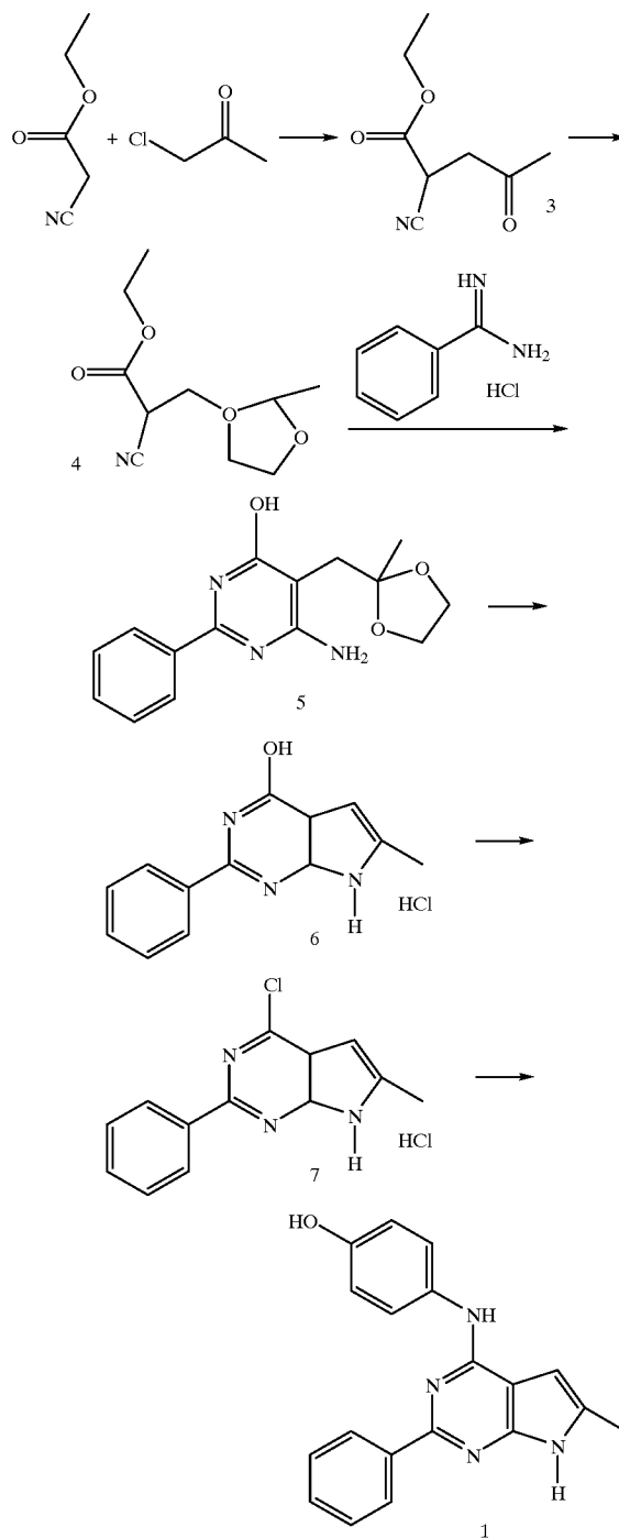
Scheme IV
