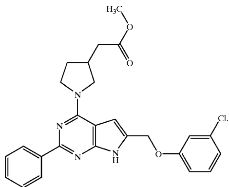
(Compound 1716)
