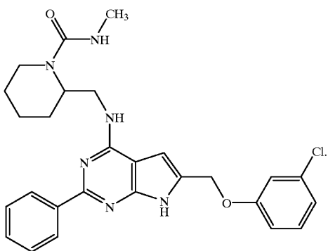
(Compound 1715)
