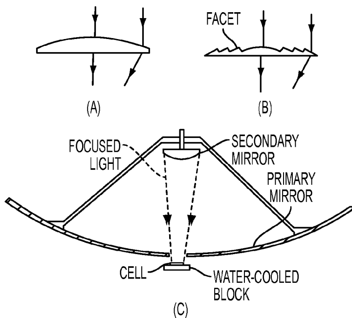
THE CONCEPTUAL LENS AND LIGHT CONCENTRATOR APPARATUS
