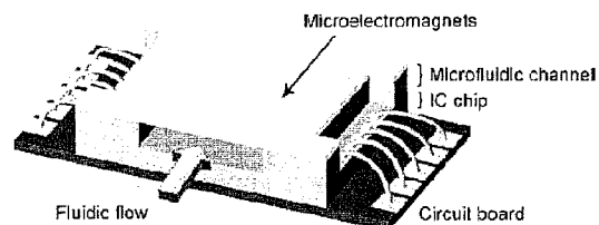
Fig. 8a. The conceptual hybrid IC and bio-lab system
