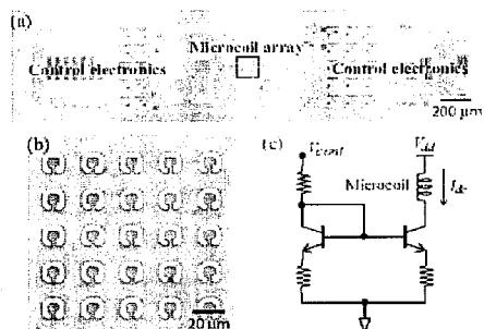
Fig. 8c. The chip and coil implementations
