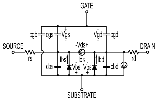
MOS TRANSIENT EQUIVALENT CIRCUIT
