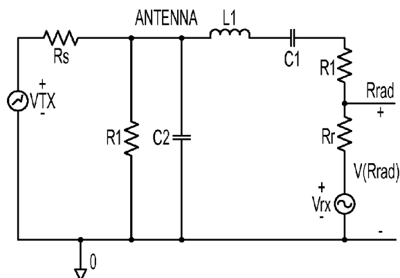
ELECTRICAL EQUIVALENT OF A HALF WAVELENGTH DIPOLE ANTENNA CONNECTED TO A-50 OHM SOURCE
