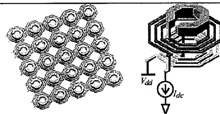
Fig. 8b. The coil array and coil layout
