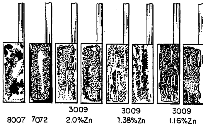
Photograph of Anode Alloy Specimens After Exposure to Galvanic Test
