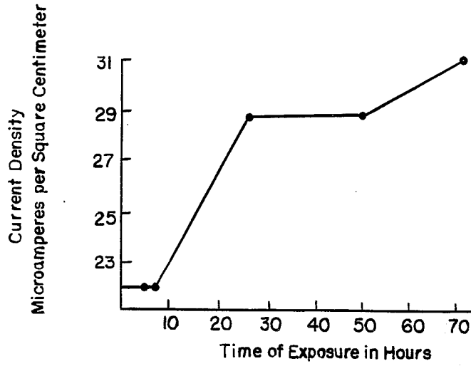
Galvanic Test on Experimental 0.86% Zinc Alloy
