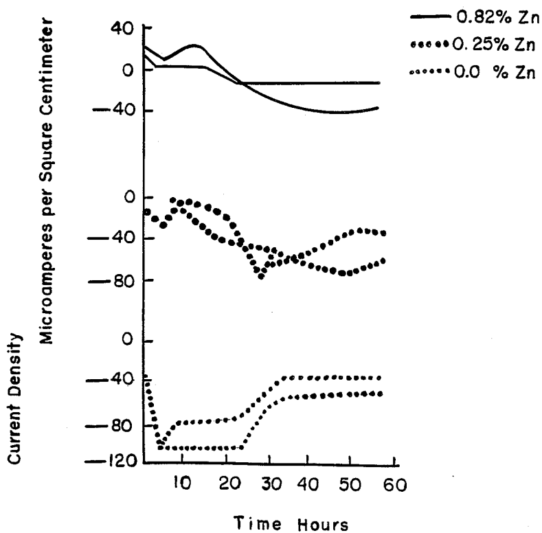
Galvanic Tests on Terre Haute Produced Materials
