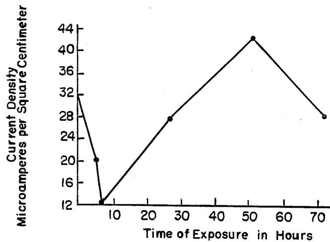
Galvanic Test on 8007 Alloy
