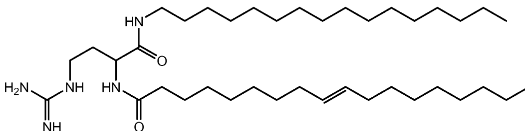
Compound 10
