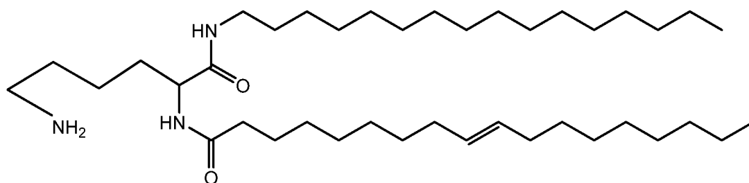
Compound 27
