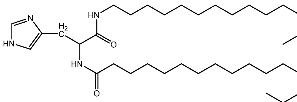
Compound 42
