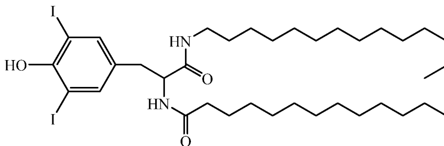
Compound 2
