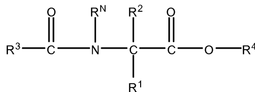
Structure 1B
