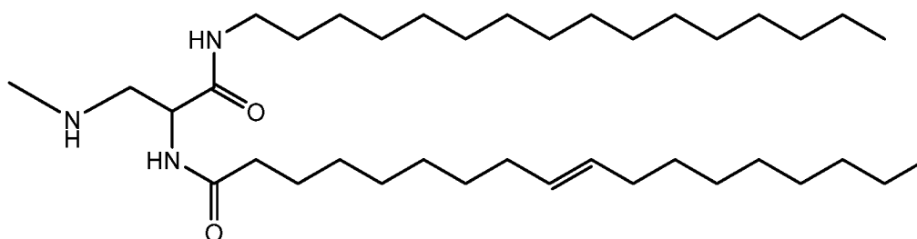
Compound 22
