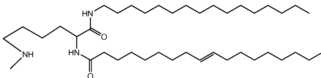
Compound 28
