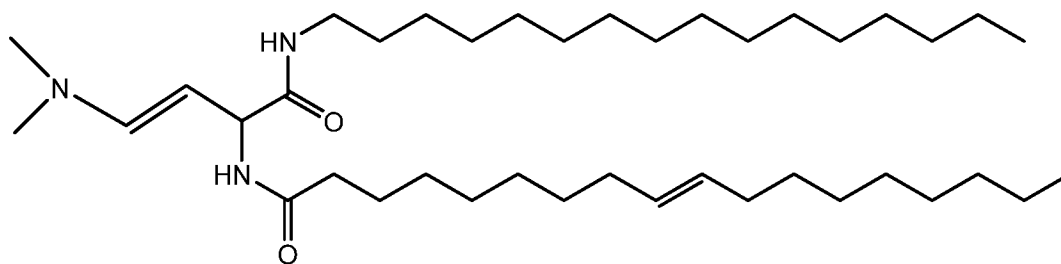
Compound 40
