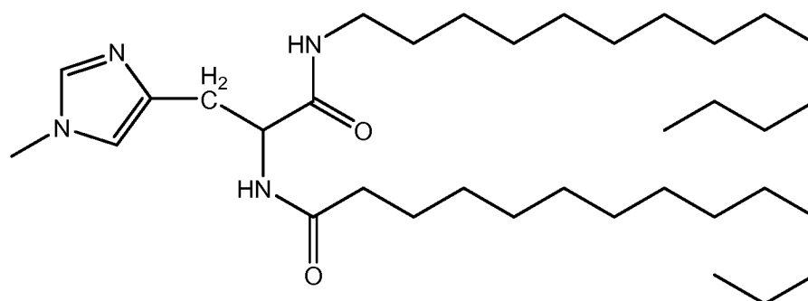
Compound 43
