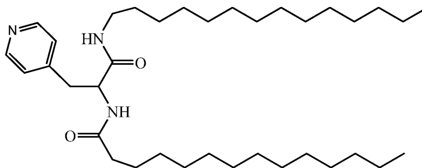
Compound 25
