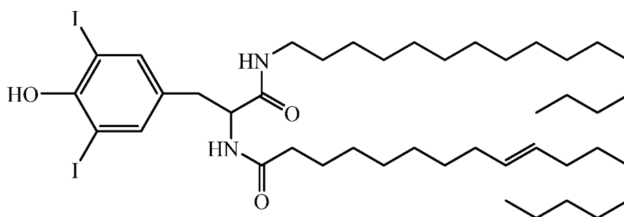
Compound 1
