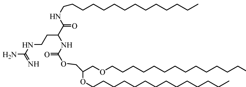
Compound 7
