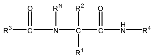
Structure 1A
