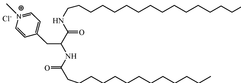
Compound 26
