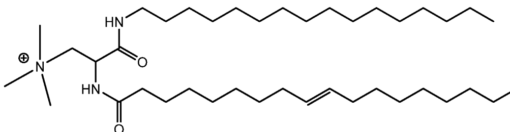
Compound 24
