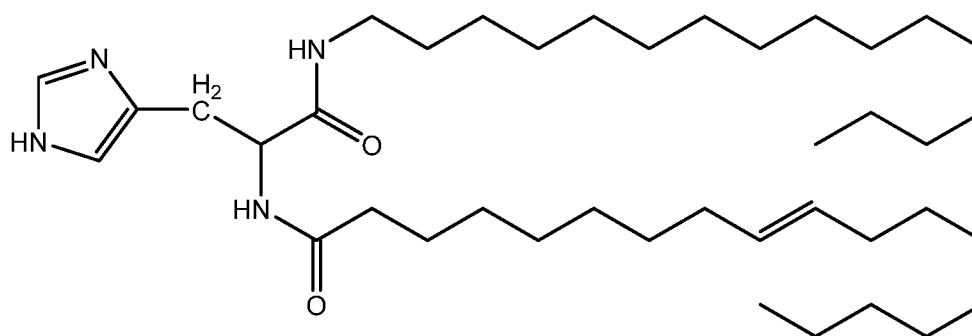
Compound 47
