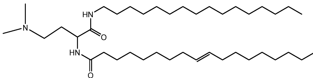
Compound 37
