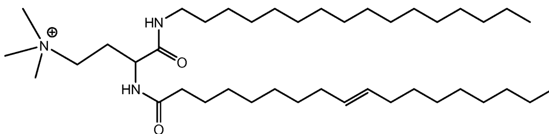
Compound 39
