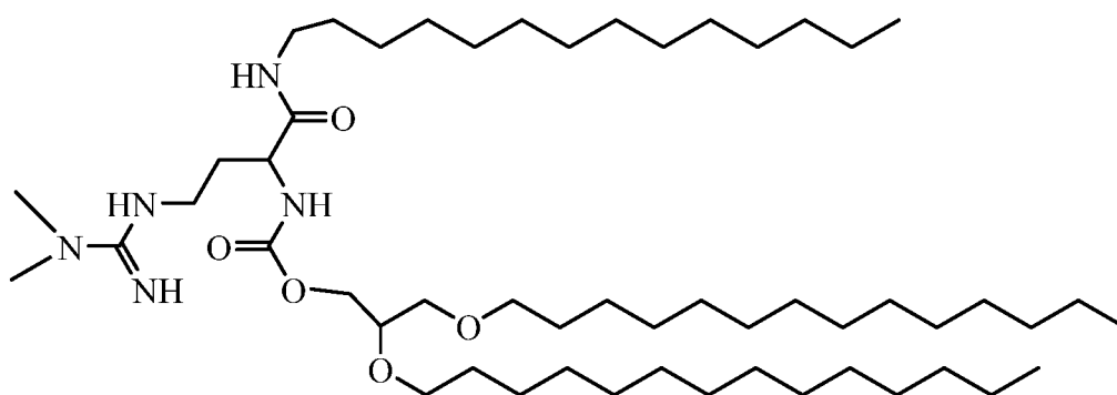
Compound 9
