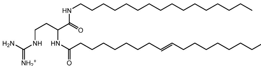
Compound 11
