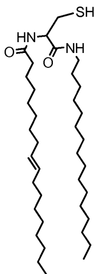
Compound 48
