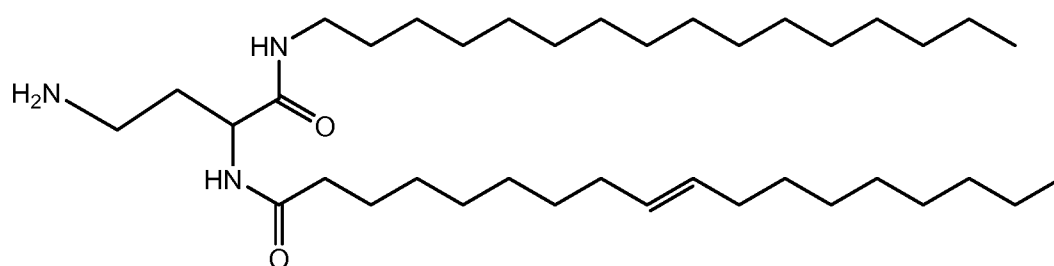
Compound 35
