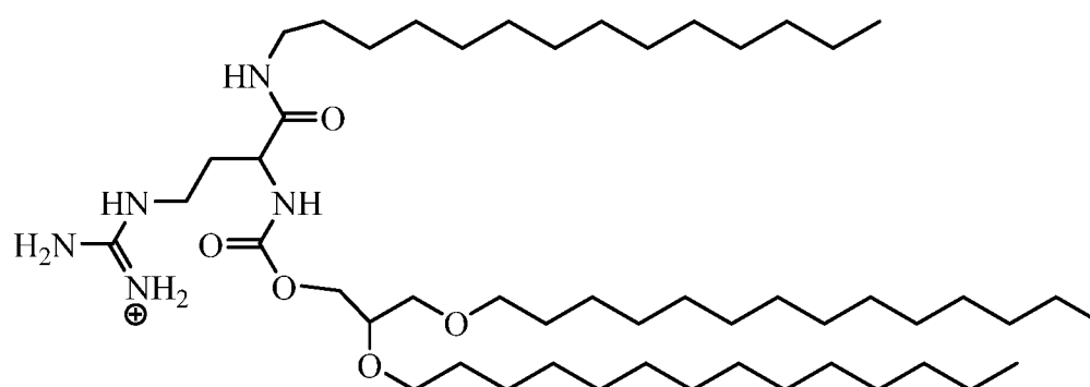
Compound 8
