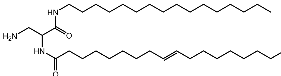
Compound 21
