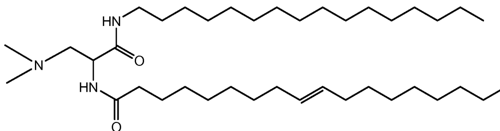
Compound 23
