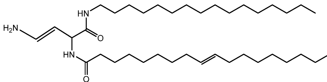
Compound 40
