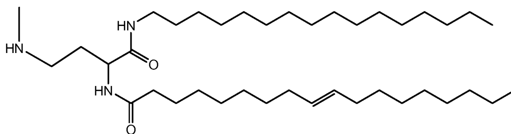
Compound 36
