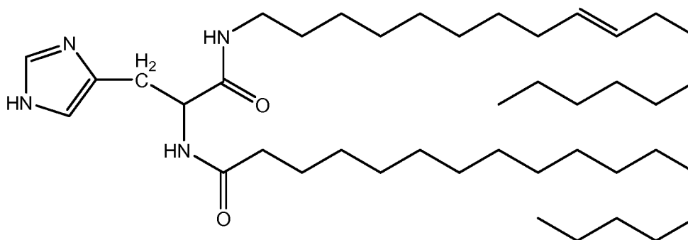
Compound 41
