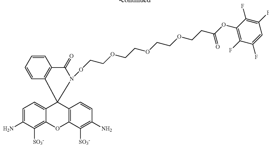
Compound I
