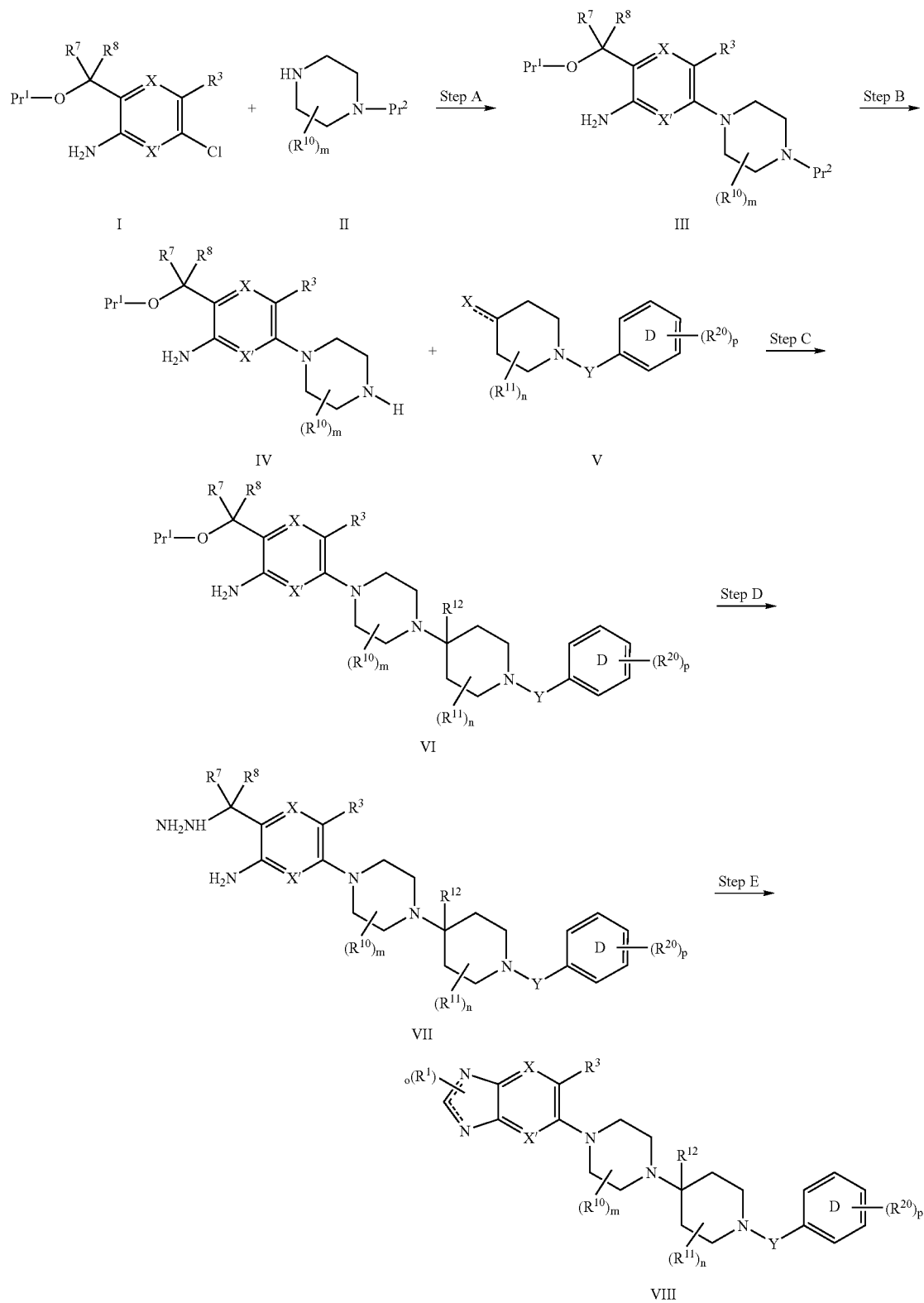
Scheme 1. Method A
