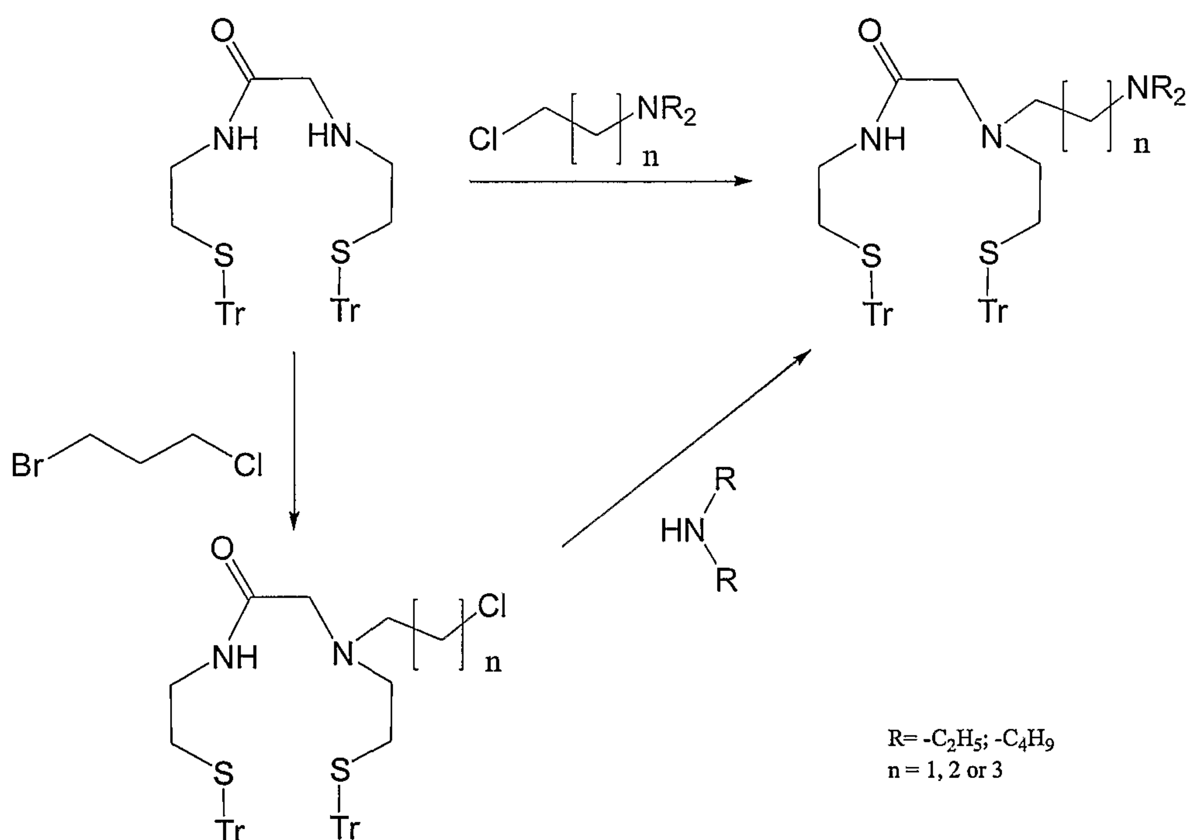
Scheme 1. Synthesis of amino-amido-dithiolate ligands.
