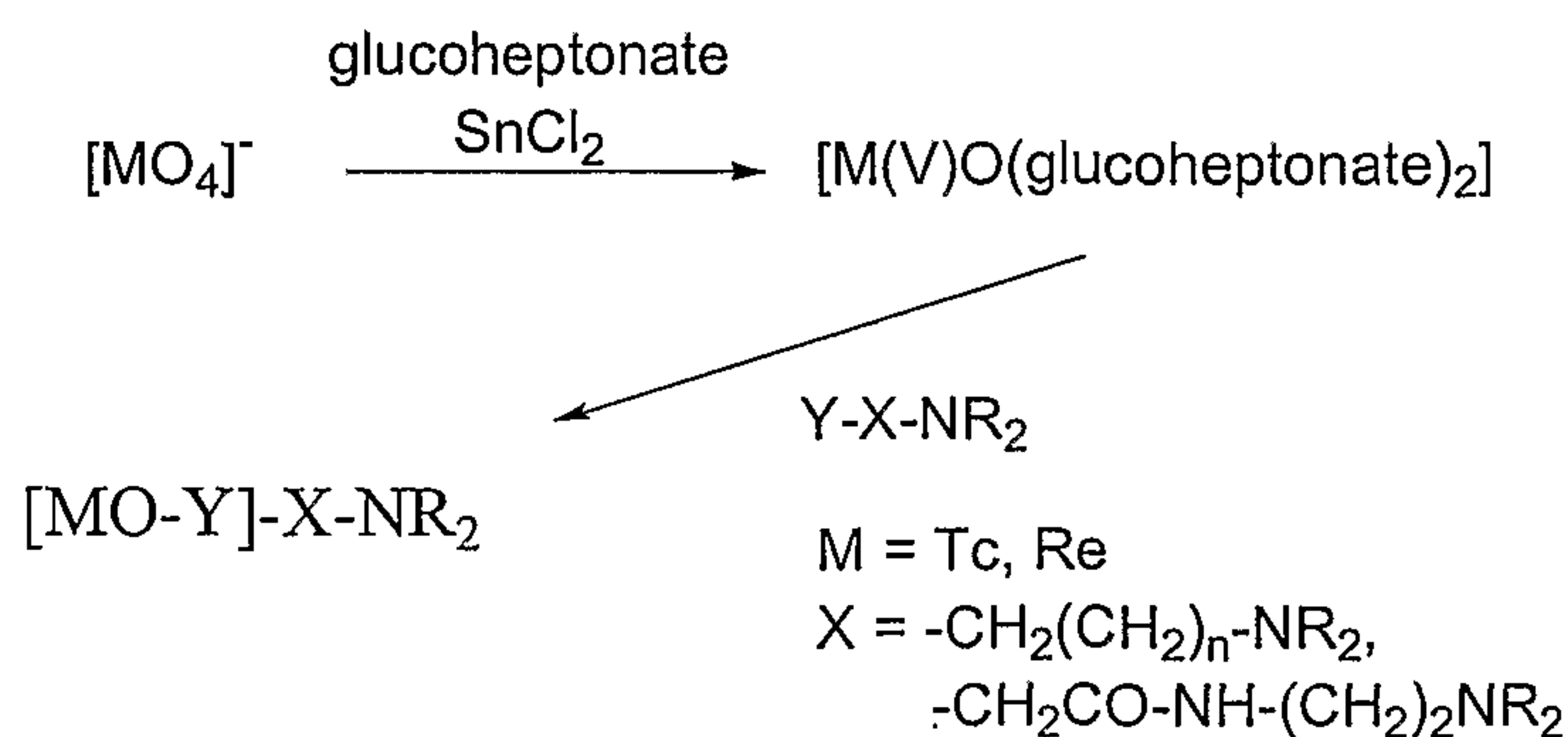
15 Scheme 2. Synthesis of metal complexes of the invention by transmetallation.
