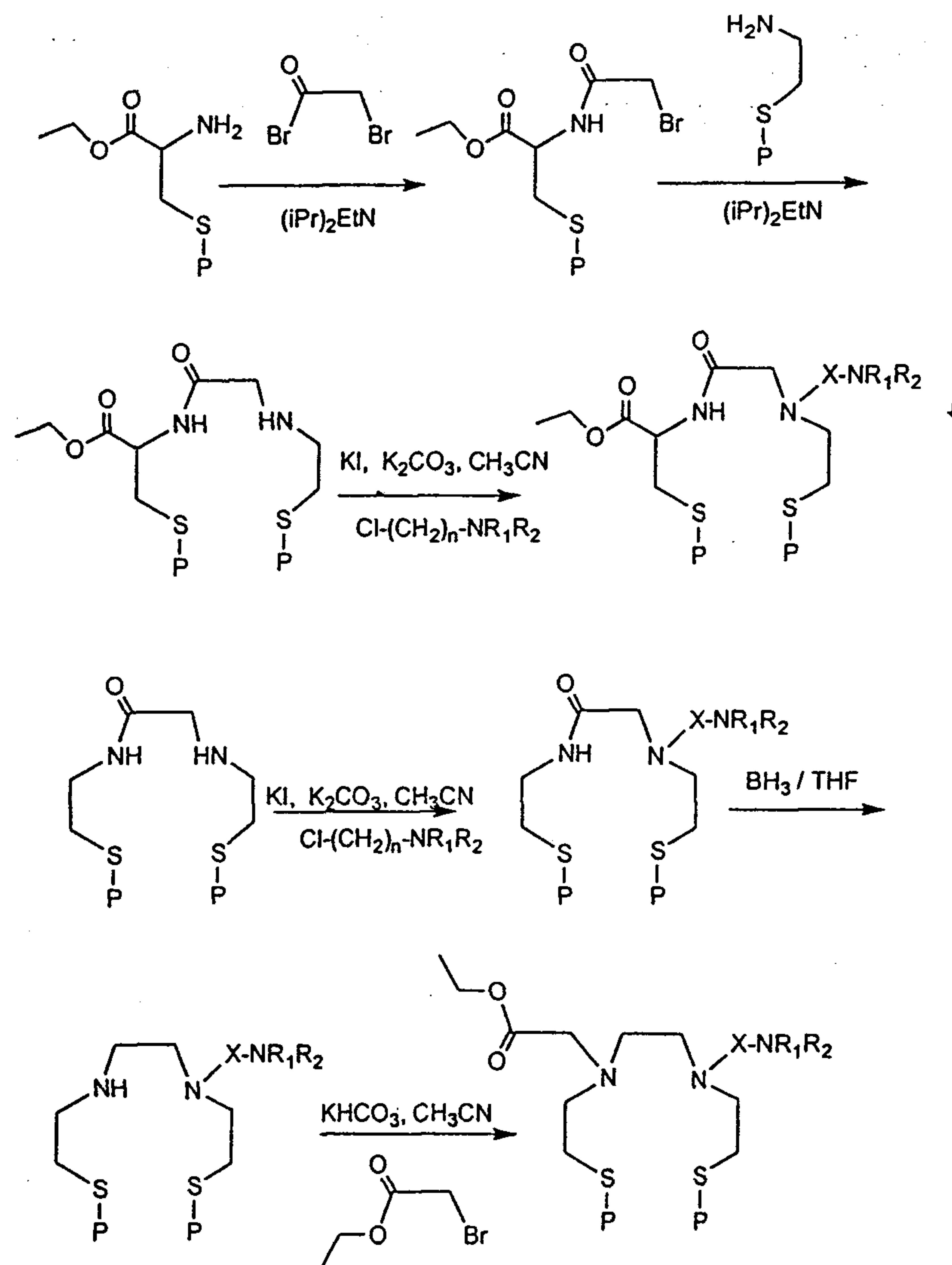
Scheme 3. Synthesis of the AADT tetradentate ligand.
