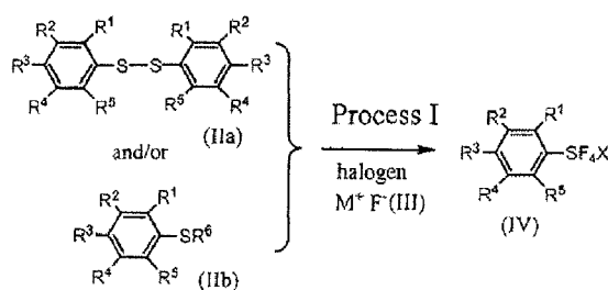
Scheme 7 (Process I)
