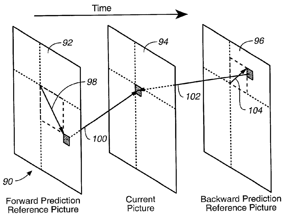
Motion Compensated Prediction and Reconstruction
