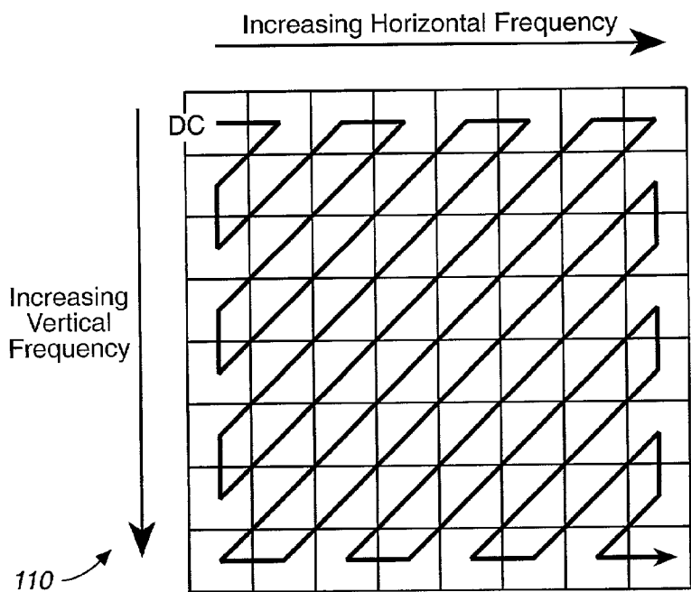
Zigzag Scanning Order of Coefficients
