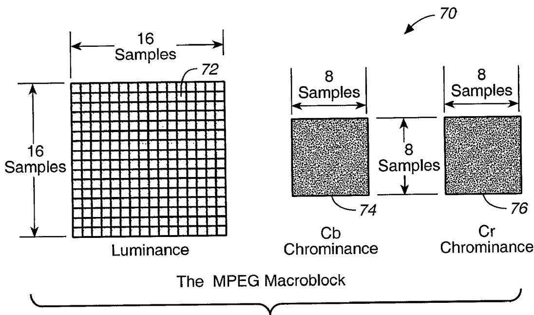
FIG._4 (PRIOR ART)
