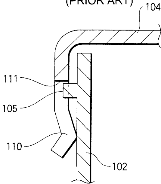
FIG.6 (PRIOR ART)
