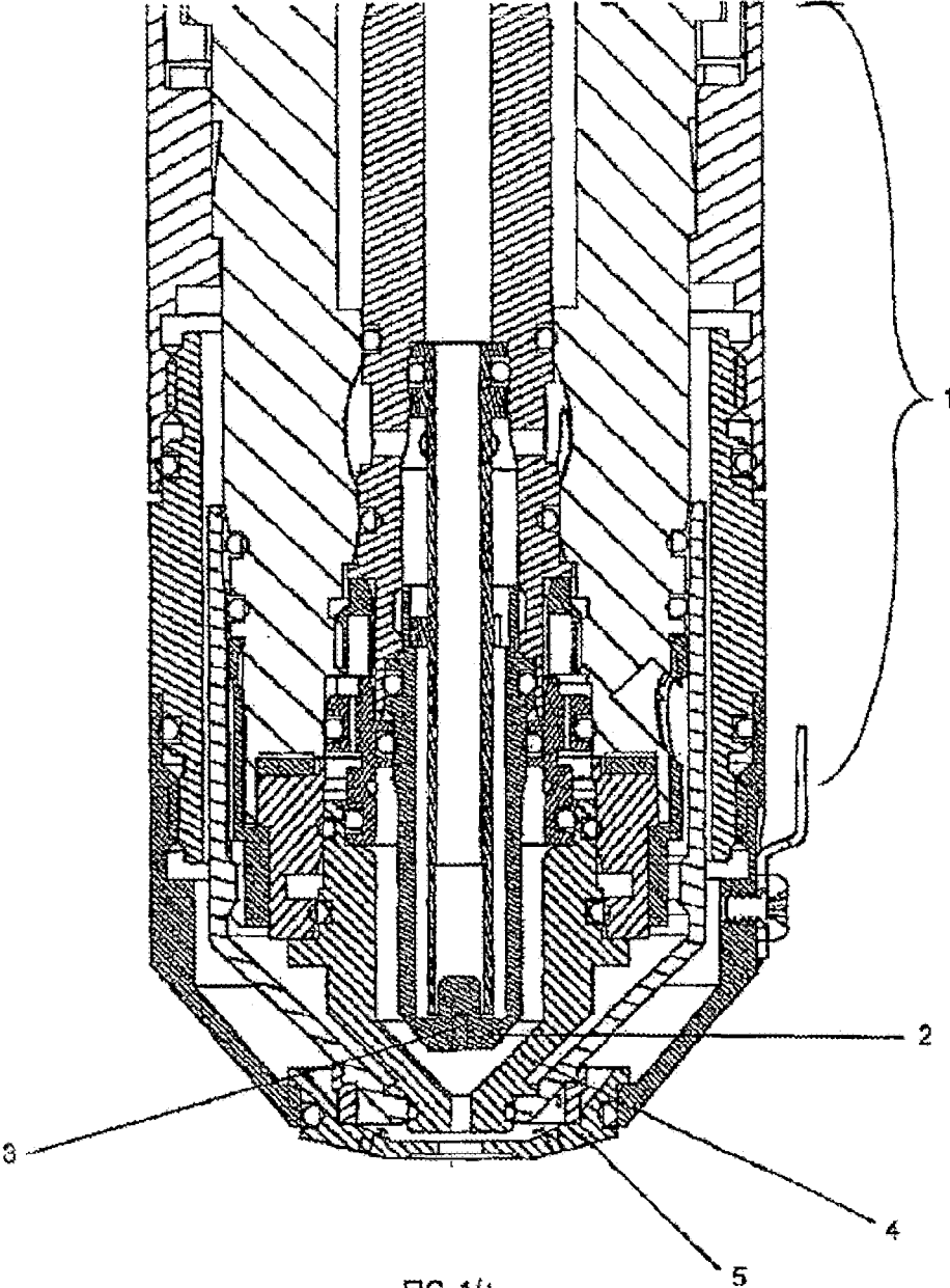
FIG. 14 (PRIOR ART)
