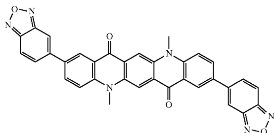
[Chemical Formula 2g]
