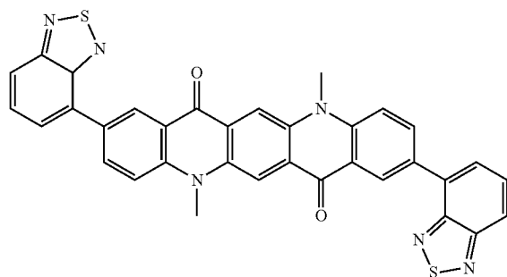
[Chemical Formula 2e]
