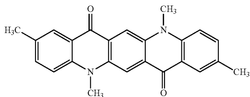
[Chemical Formula 2b]
