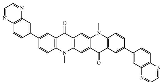
[Chemical Formula 2h]
