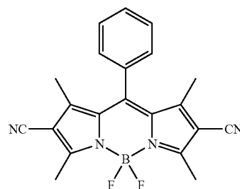
[Chemical Formula 1d]
