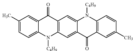
[Chemical Formula 2e]
