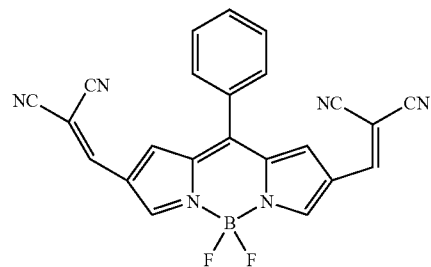
[Chemical Formula 1i]
