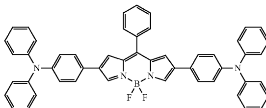
[Chemical Formula 1h]
