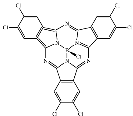
[Chemical Formula 3c]
