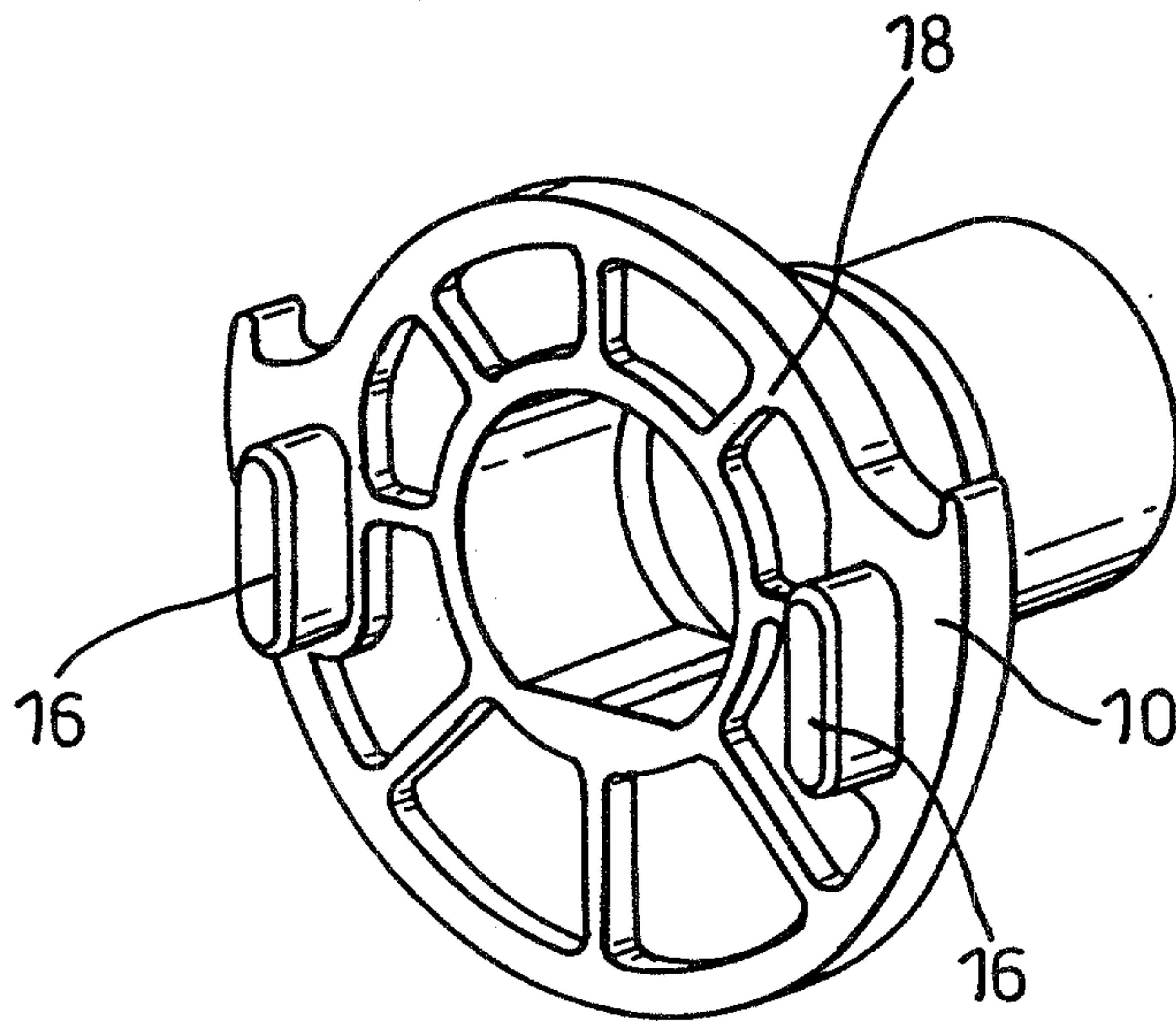
Fig. 1c (PRIOR ART)
