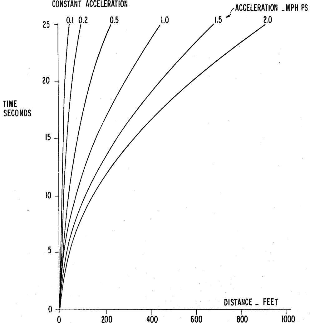
FIG. 11 TIME TO REACH CROSSING VERSUS DISTANCE FROM CROSSING AT WHICH MOTION BEGINS WITH CONSTANT ACCELERATION
