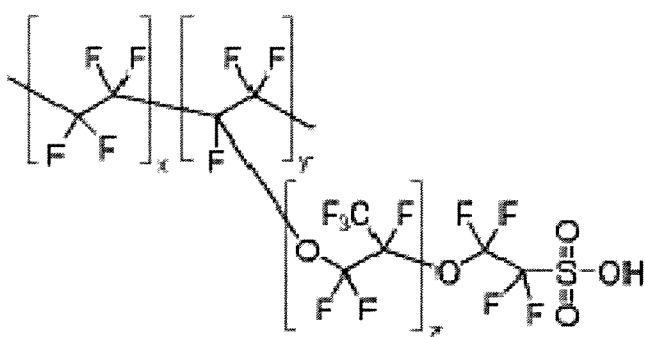
Diagram 2. Structure of Perfluorinated Sulfonic Acid Resin Catalysts.
