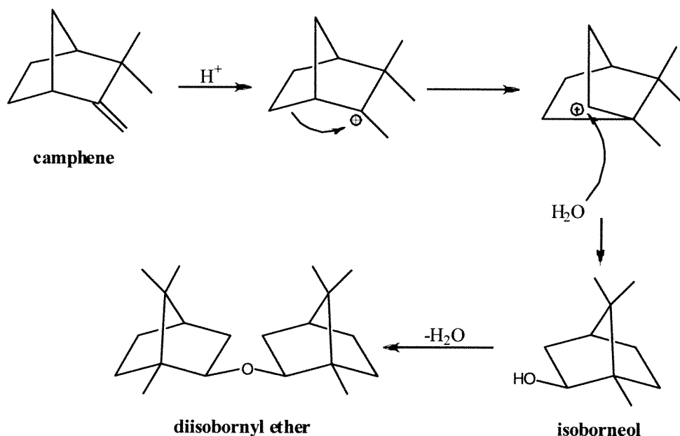
Scheme 6. Acid catalyzed conversion of camphene to diisobornyl ether.
