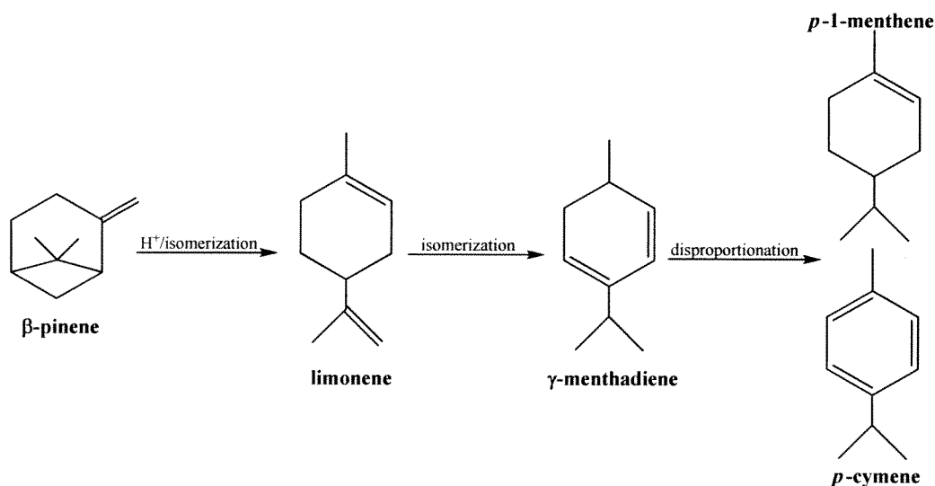
Scheme 2. Potential mechanism for the conversion of \beta -pinene to p -cymene.
