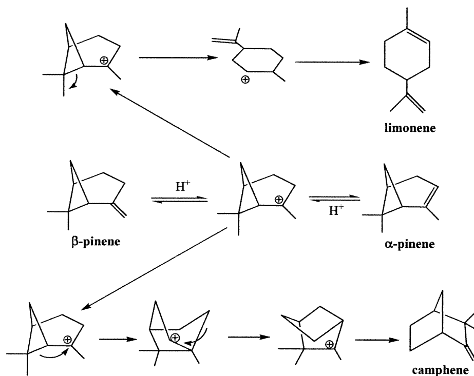
Scheme 1. Mechanism for the isomerization of \beta -pinene over MMT-K10.
