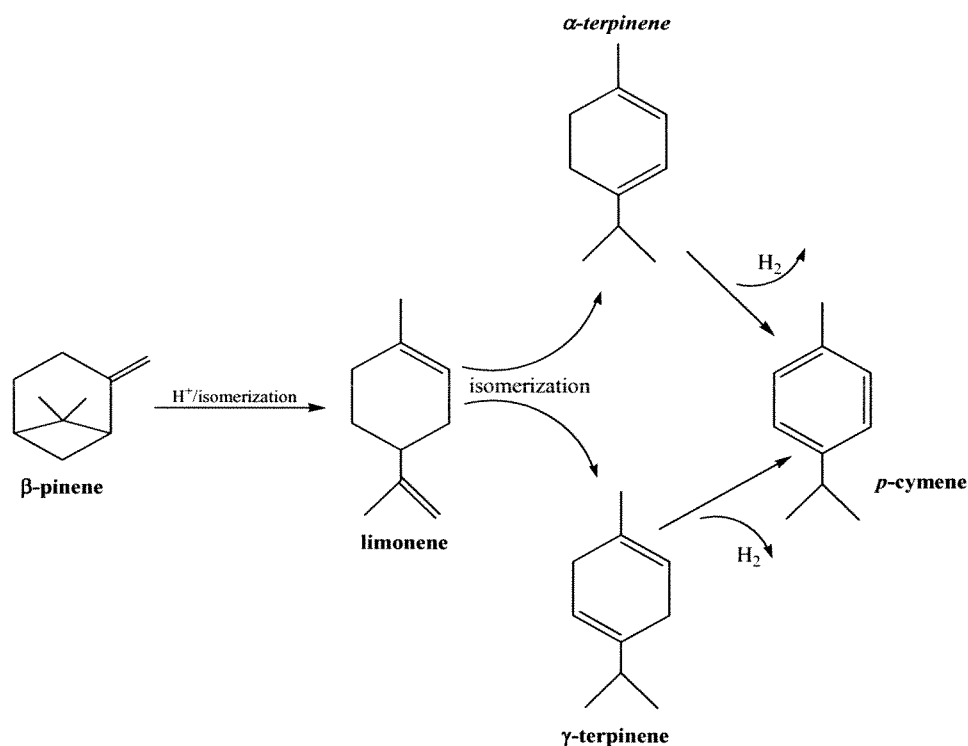
Scheme 3. Potential mechanism for the conversion of \beta -pinene to p -cymene.
