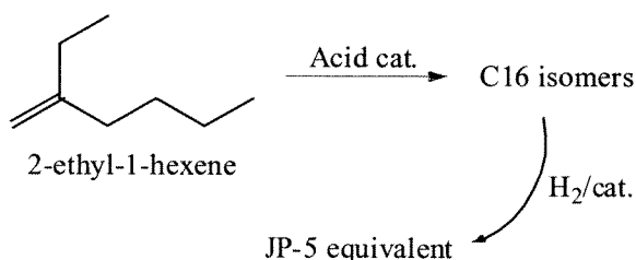
Scheme 10. Acid catalyzed dimerization of 2-ethyl-1-hexene for the synthesis of renewable jet fuel.
