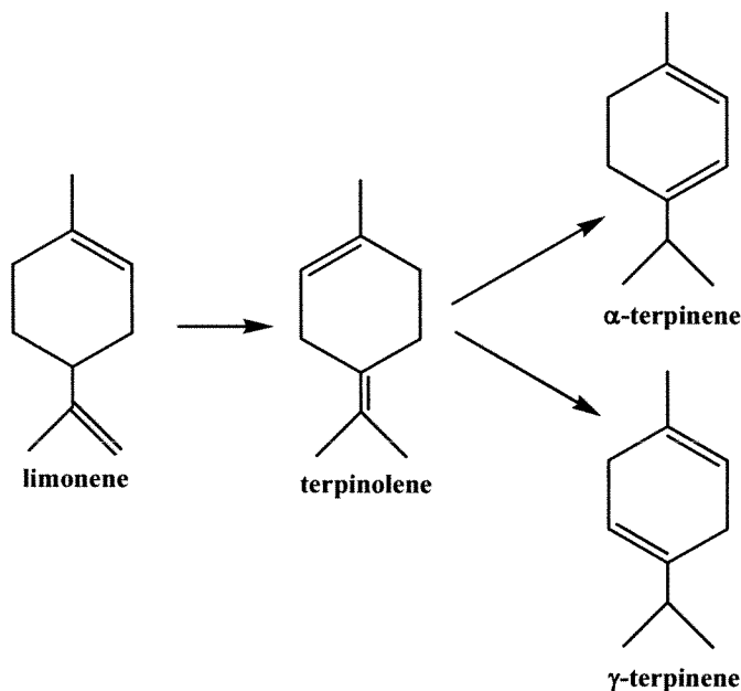
Scheme 4. Stepwise conversion of limonene to terpinenes through terpinolene.
