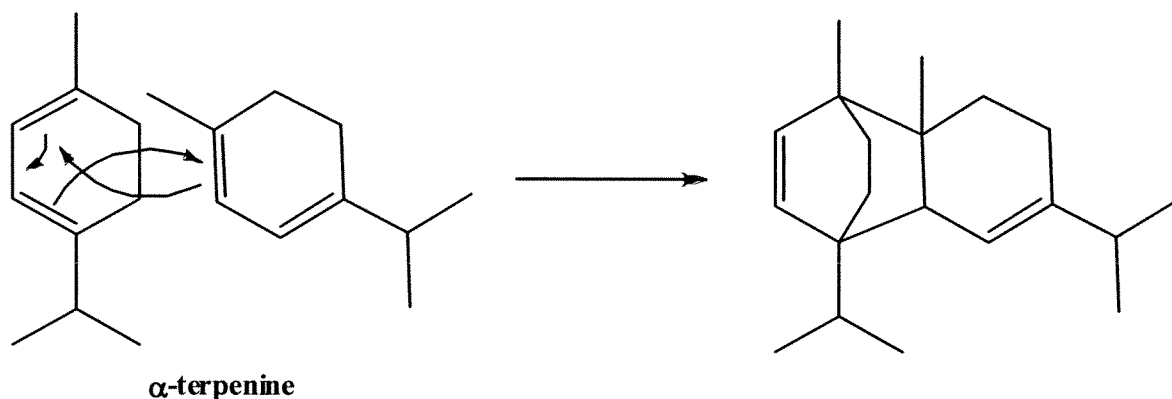
Scheme 5. Example of a potential Diels Alder dimerization reaction of \alpha -terpinene.
