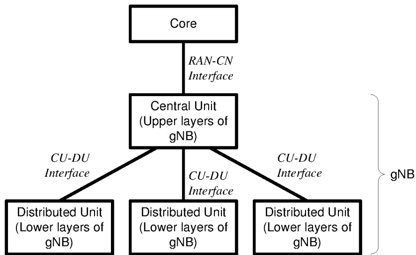
FIG. 13B Centralized deployment
