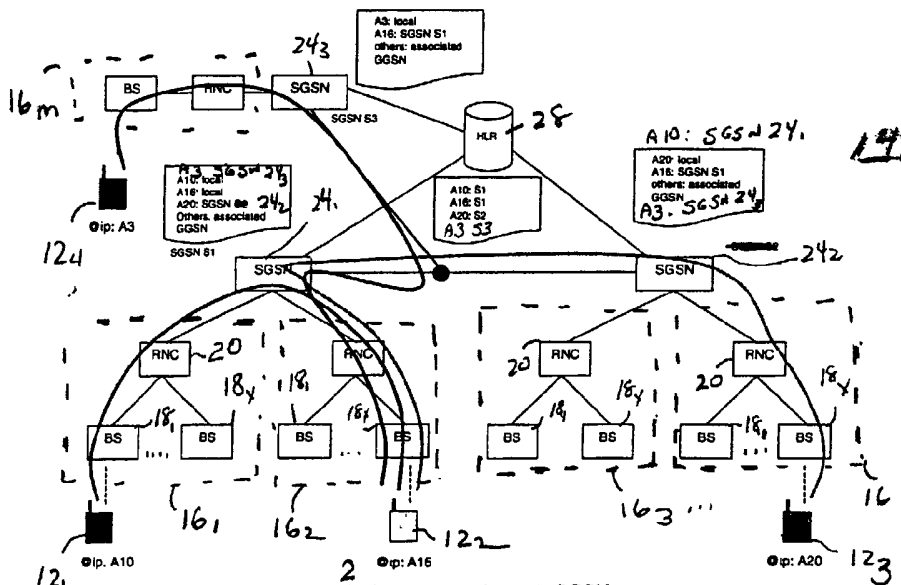
Figure 3 - IP sessions through SGSNs
