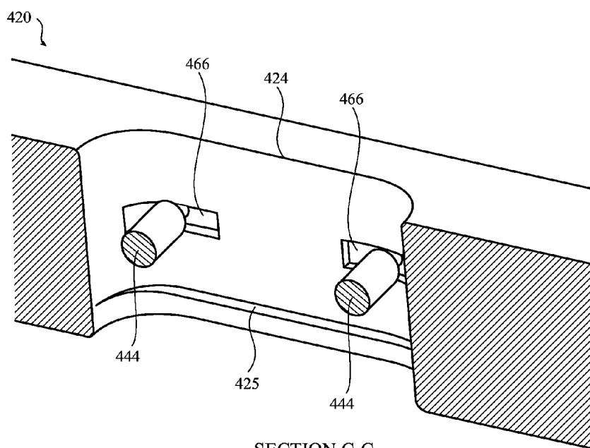
SECTION C-C FIG. 9B
