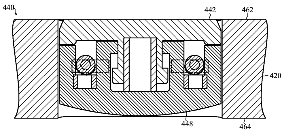
SECTION C-C FIG. 10B
