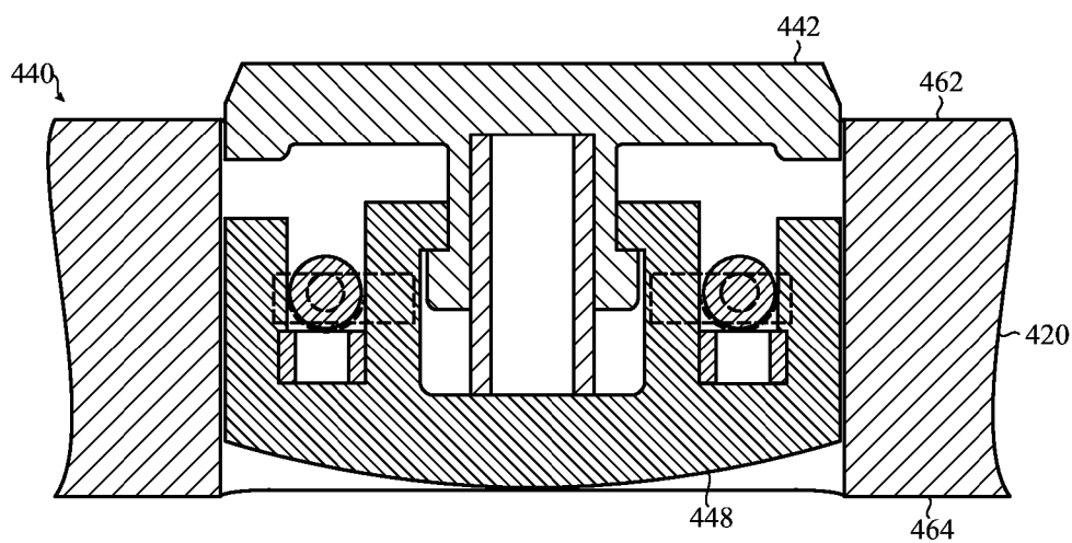
SECTION C-C FIG. 10C
