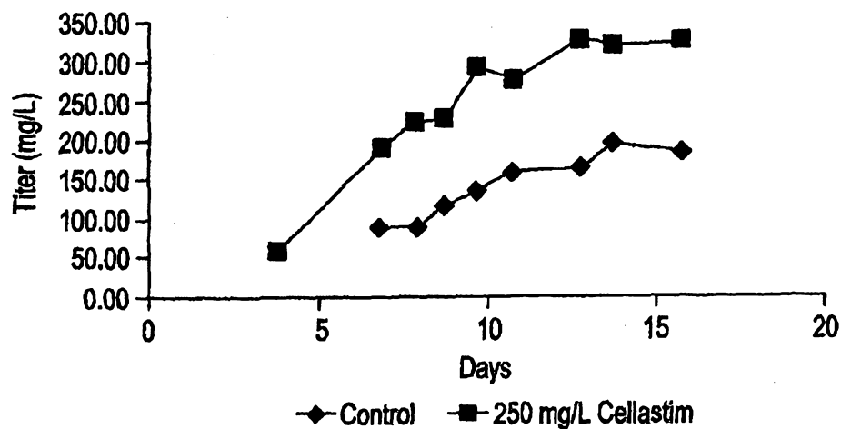
FIG. 16A Product Concentrations EXP 4 Bioreactors
