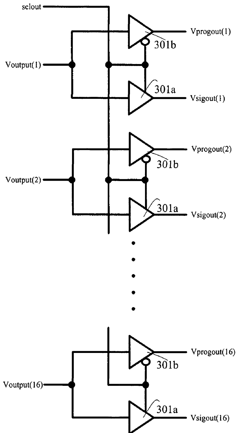
Fig.3 Output Selector Circuit
