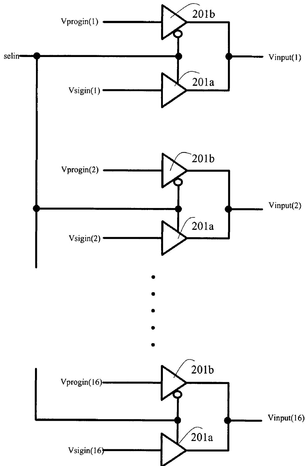
Fig.2 Input Selector Circuit
