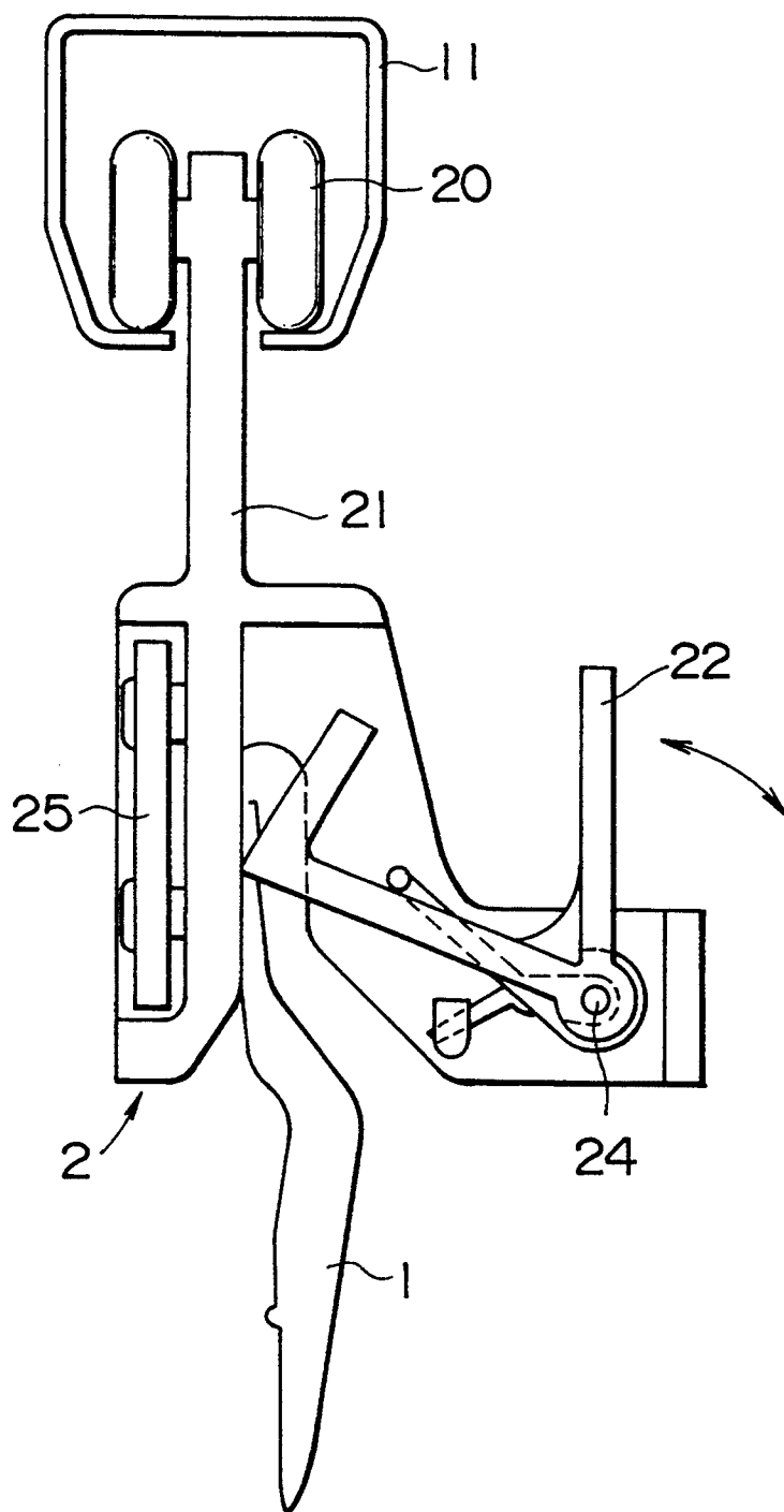
FIG. 15 RELATED ART
