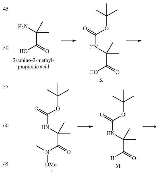
Scheme 7. Alternative exemplary synthesis of intermediate J.
