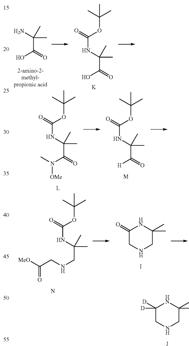
Scheme 11. Synthesis of intermediate J.
