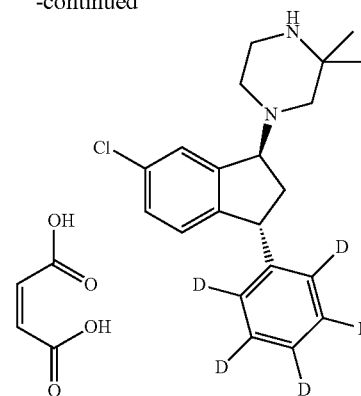
(XXV) maleate Mw 462.00 (345.93 + 116.07) trans racemate (+8% cis)
