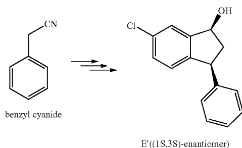
Scheme 4. Exemplary synthesis of intermediates E and E'.
