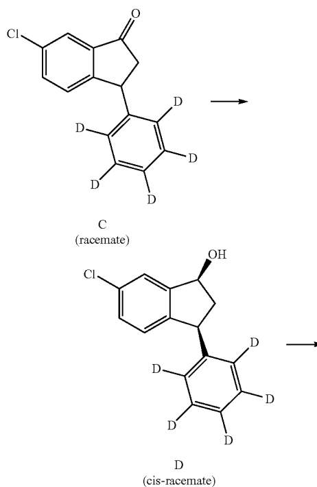
Scheme 2. Exemplary synthesis of intermediate E.
