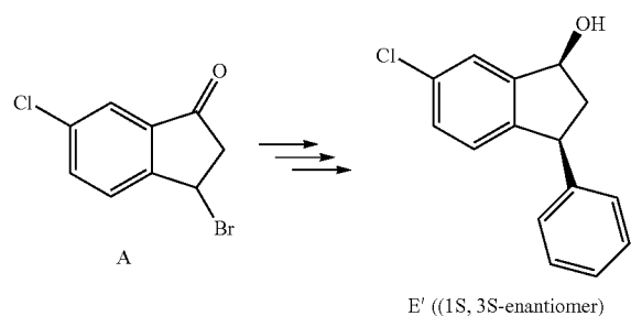
Scheme 3. Exemplary synthesis of intermediate E'.
