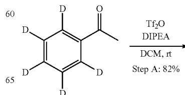
Scheme 14. Synthesis of Compound (XV)
