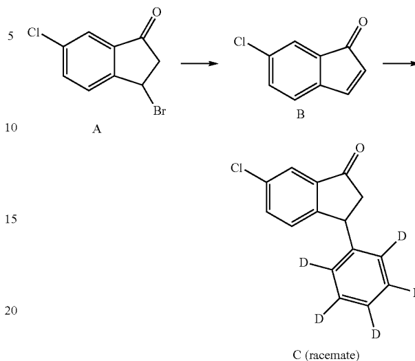
Scheme 1. Exemplary synthesis of intermediate C.
