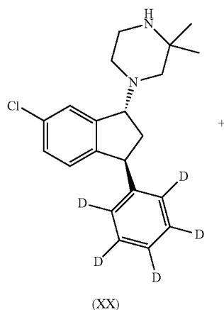
Scheme 17: Synthesis of rac-trans-1-(6-chloro-3-phenyl(d 3 )-indan-1-yl)-1-(d 3 ), 2,2-trimethyl-piperazine succinate
