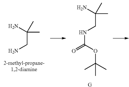
Scheme 6. Exemplary synthesis of intermediate J.
