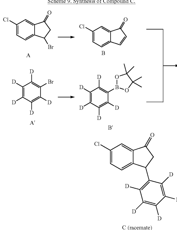
Scheme 9. Synthesis of Compound C.
