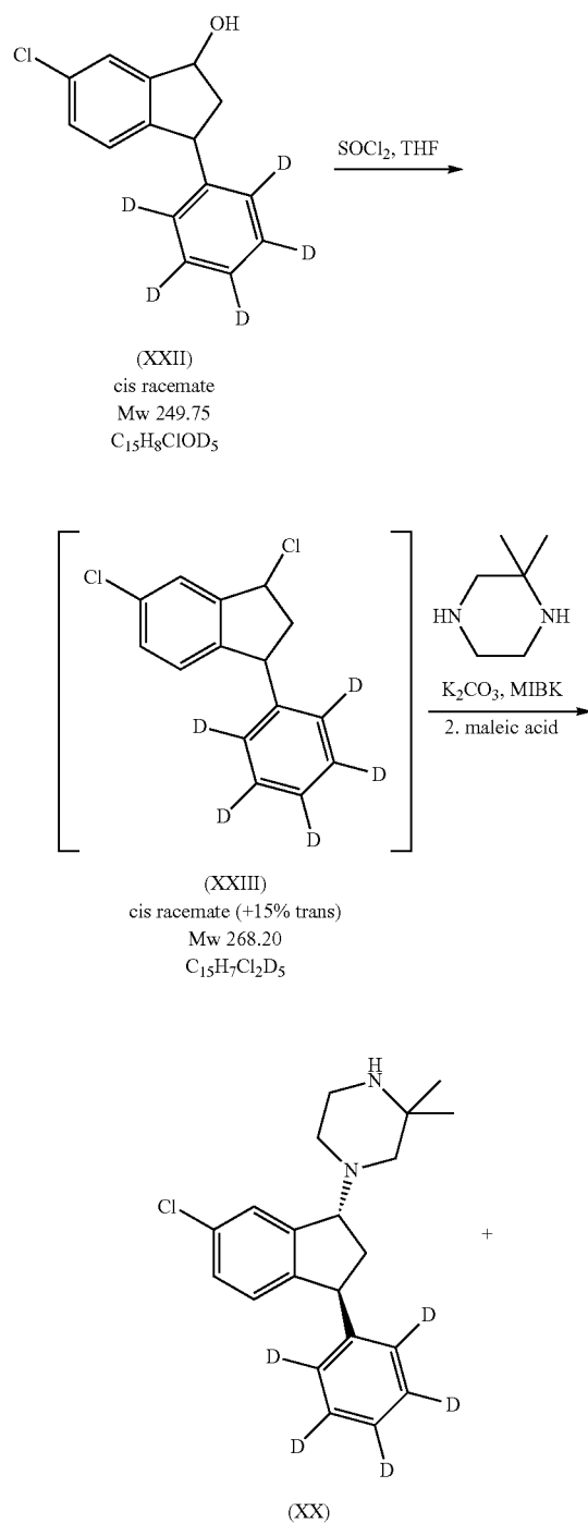
Scheme 16: Synthesis of rac-trans-1-(6-Chloro-3-phenyl( d_5 )-indan-1-yl)-3,3-dimethyl-piperazine maleate
