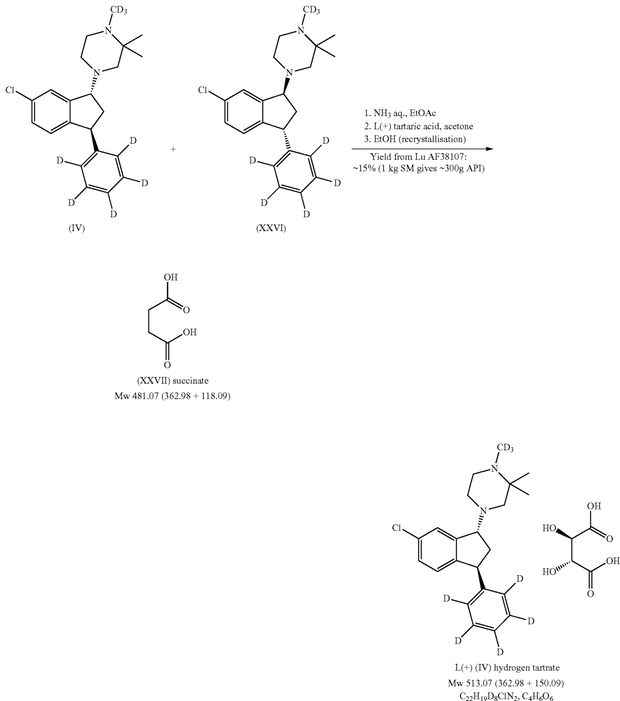
Scheme 18: Synthesis of 4-((1R, 3S)-6-chloro-3-phenyl(d 3 )-indan-1-yl)-1-(d 3 ),2,2-trimethyl-piperazine L(+)-hydrogen tartrate.
