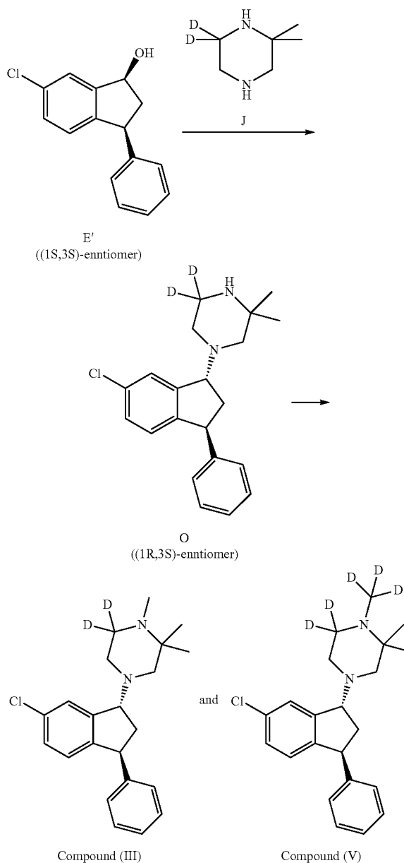
Scheme 12. Synthesis of Compound (III) and Compound (V).
