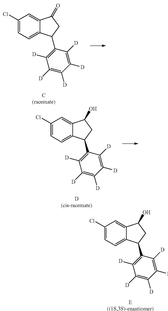
Scheme 10. Synthesis and resolutions of Compound E.
