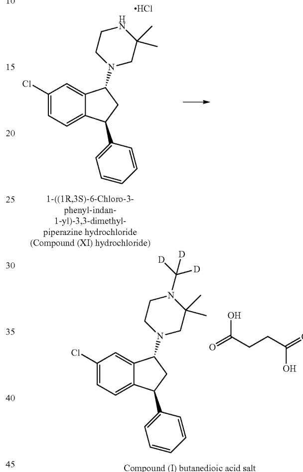
Scheme 8. Synthesis of Compound (I).
