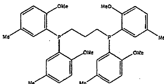
1,3-bis[bis(2-methoxy-5-methylphenyl)phosphino]propane BIBMAPP
