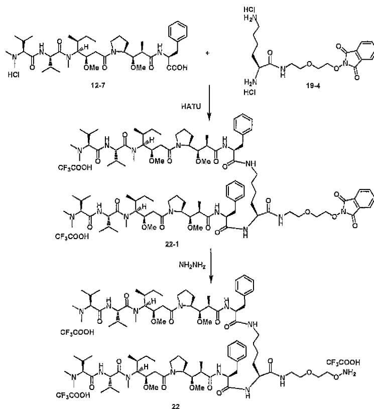
Scheme 22
