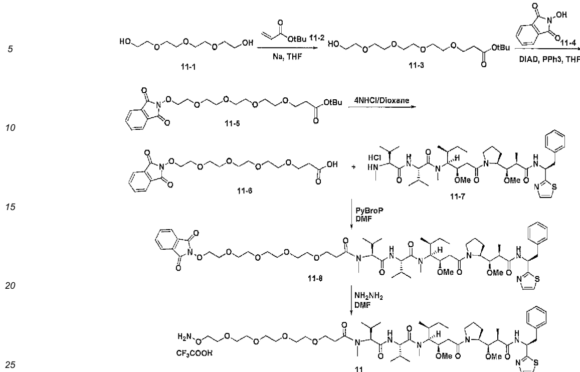
Scheme 11
