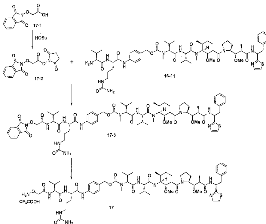
Scheme 17
