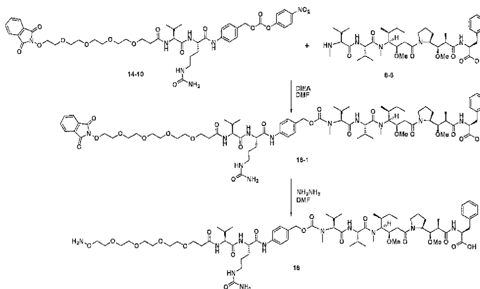
Scheme 18
