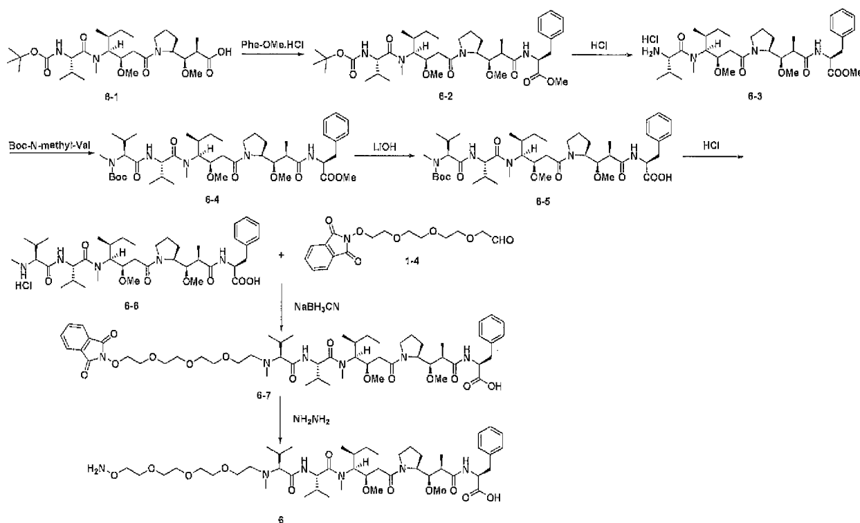
Scheme 6
