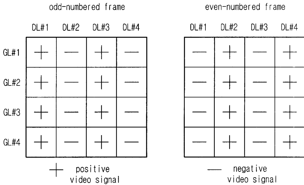
Fig.3C (Prior Art)
