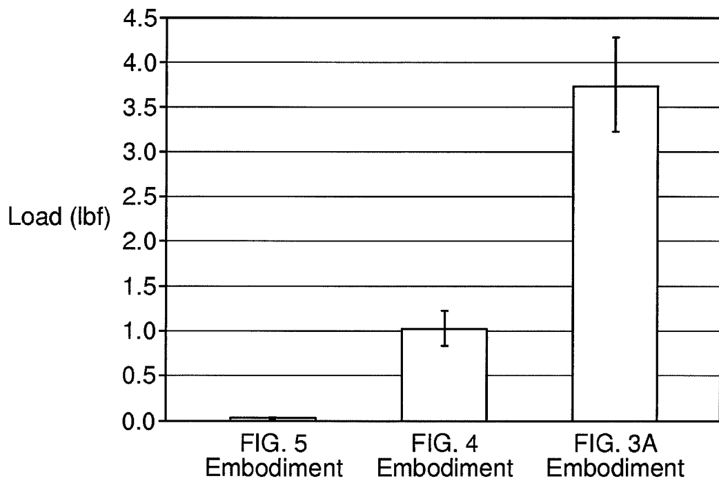
Pull-Through Pledget - Max Load at Pledget Stopper
