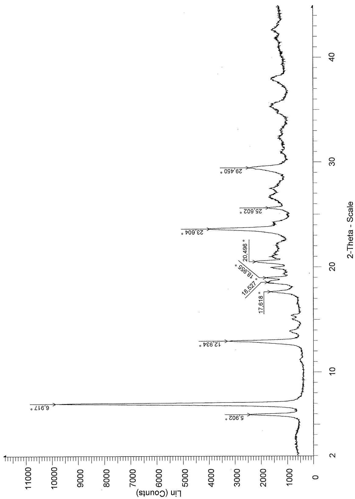
Figure 4A: Powder X-ray diffraction pattern for crystalline Dolutegravir potassium Form II.
