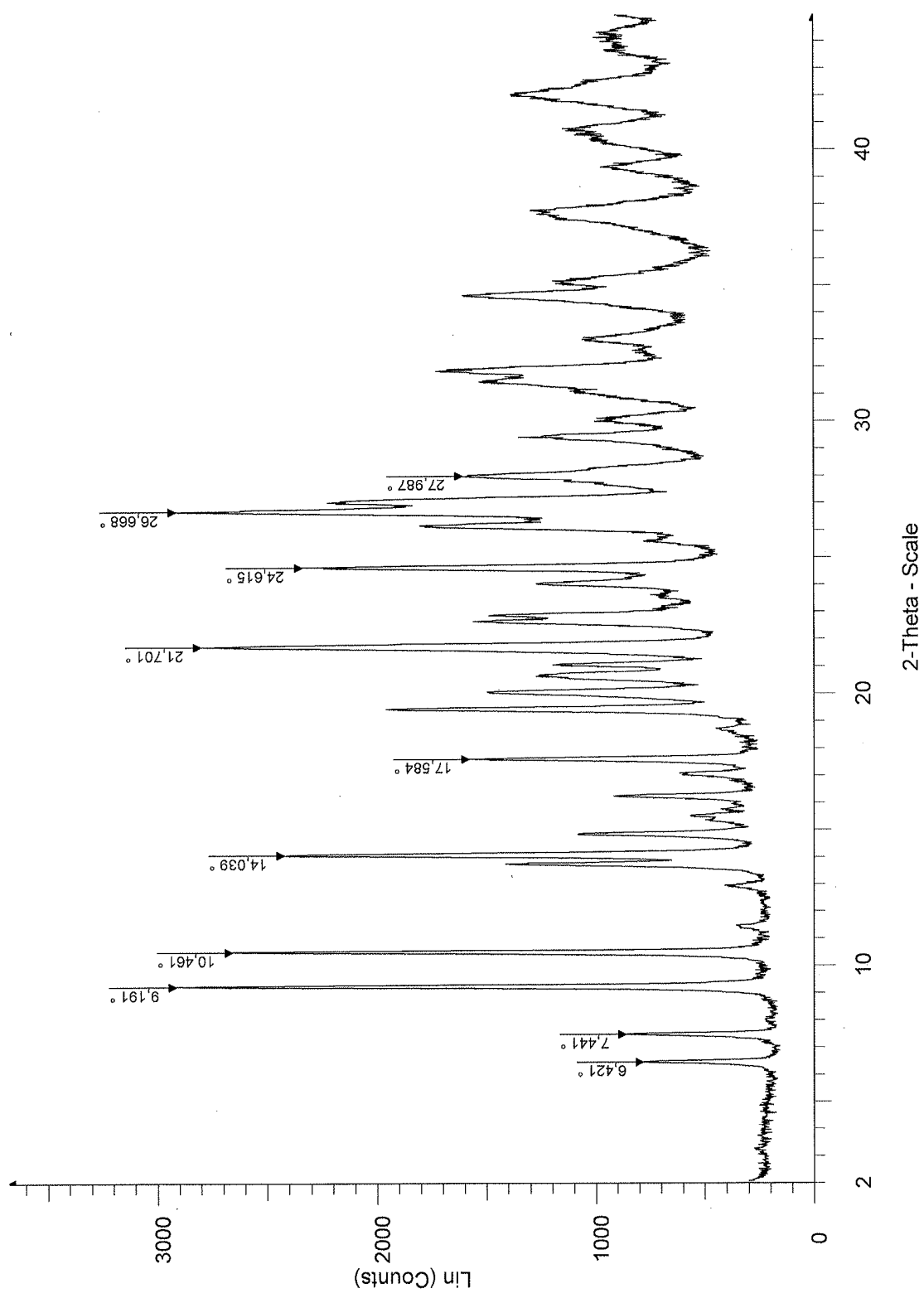
Figure 19A: powder X-ray diffraction pattern for crystalline Dolutegravir potassium Form VII.
