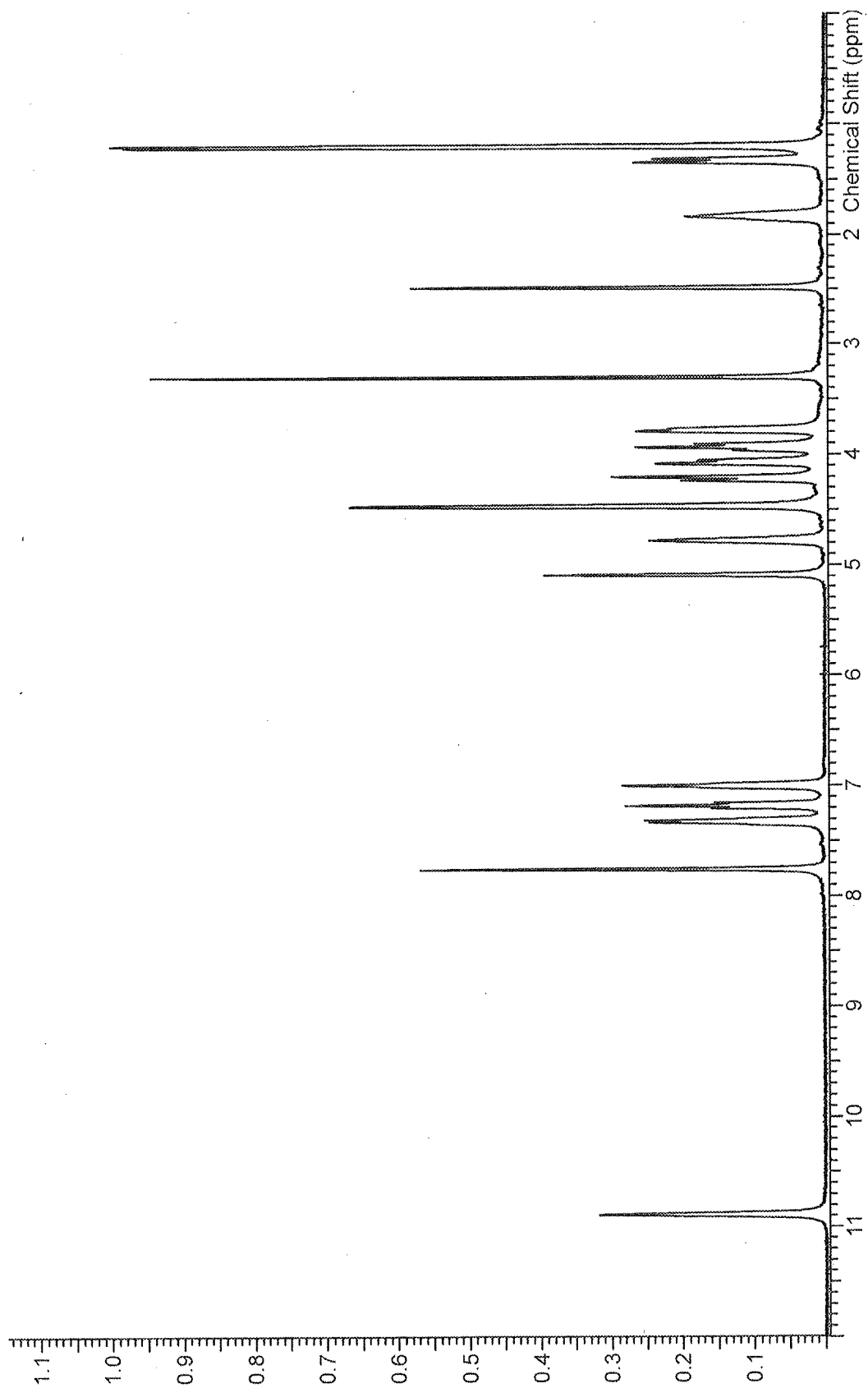
Figure 1: ^1\text{H} -NMR spectrum for Dolutegravir potassium salt.
