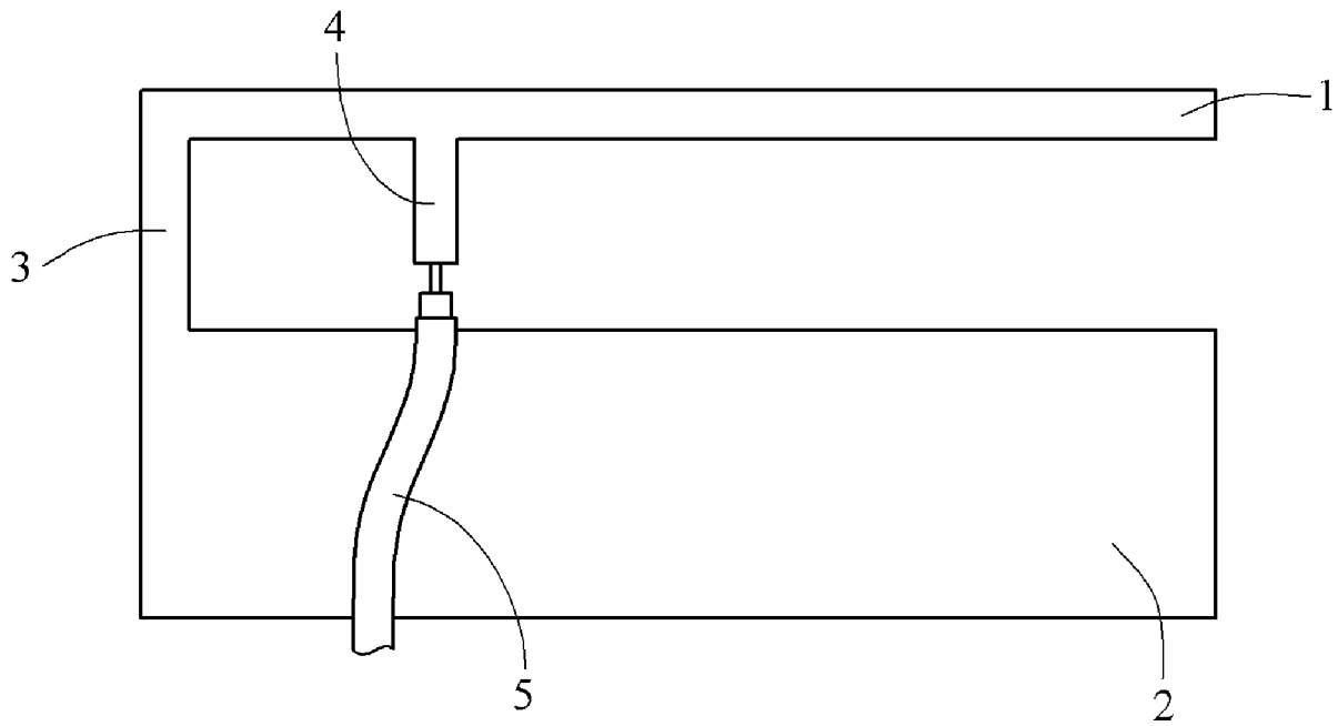
FIG. 1 (PRIOR ART)
