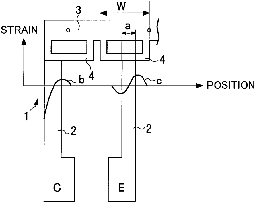
FIG. 14 PRIOR ART
